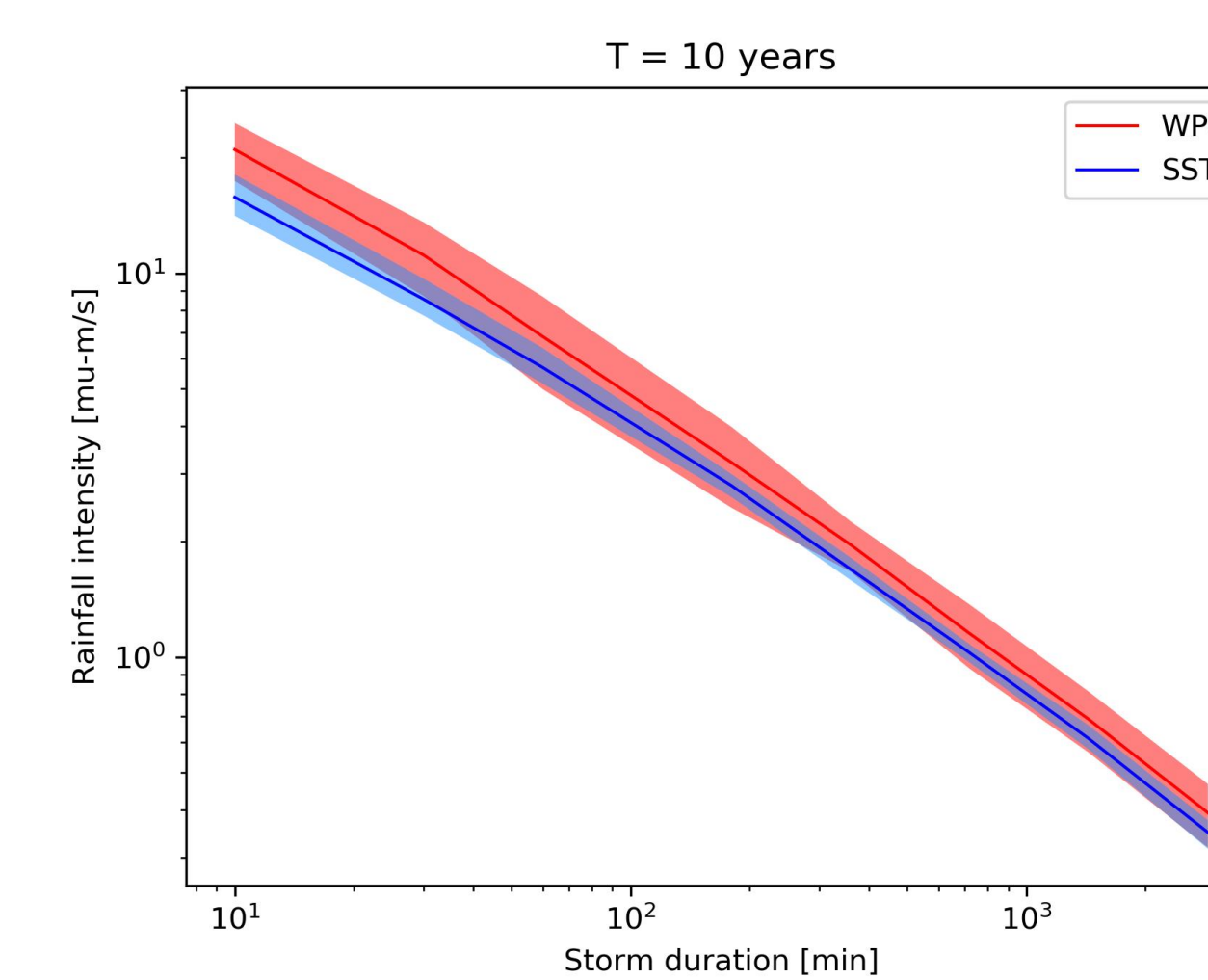
Figure #3: The danish regional model compared to IDF estimates from SST. Shaded area indicates 95% spread. WPC are IDF-curves extracted from the regional model. T indicates return level.
