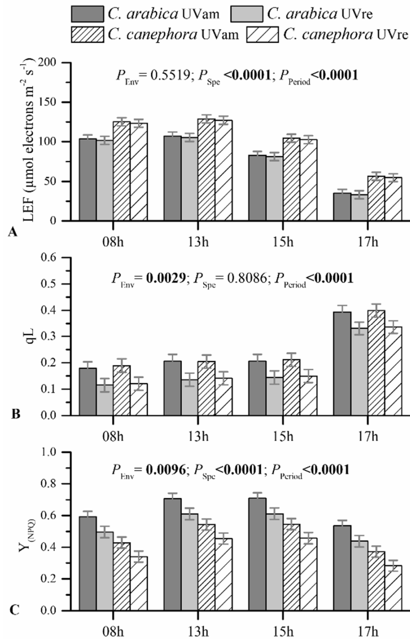
Figure 6. Linear electron transport (LEF) (A), the fraction of “open” PSII centers— q_L (B), and the yield for dissipation by downregulation— Y_{(\text{NPQ})} (C), measured in light-adapted leaves during four diurnal periods (8.00 a.m., 1.00, 3.00, and 5.00 p.m.) for Coffea arabica and C. canephora grown under near ambient (UVam) and reduced (UVre) UV levels (Env). Estimated mean values \pm S.E. ( n = 8 ) and ANOVA p -Values are shown. ANOVA p -Values < 0.05 are marked in bold.
