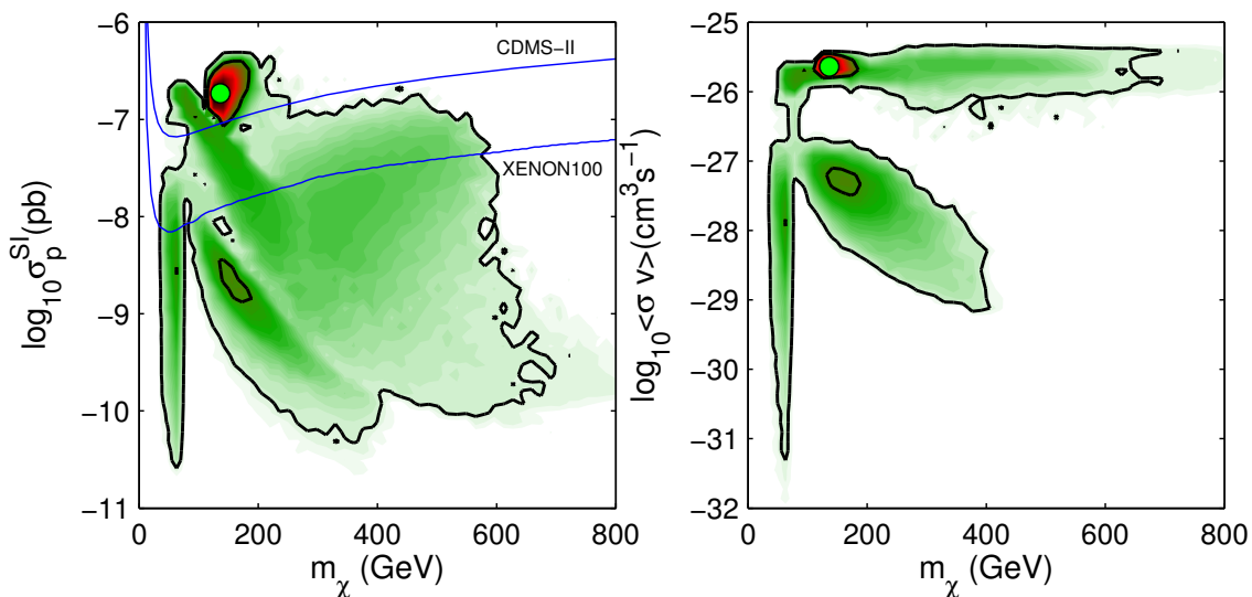
Figure 11. 2-D profile likelihood functions for flat+log merged chains for spin-independent scattering cross-section of the neutralino and a proton \sigma_p^{\text{SI}} versus the neutralino mass m_\chi (left panel) and velocity-averaged neutralino self-annihilation cross-section \langle\sigma v\rangle versus the neutralino mass m_\chi (right panel). The contours represent the 68% and 95% profile likelihood confidence intervals. 20,000 live points were used with tol set to 1 \times 10^{-4} . The best-fit parameters values are shown by green circle. The latest experimental exclusion limits at the 90% confidence level from CDMS-II [41] and XENON100 [42] are also shown in the left panel.
