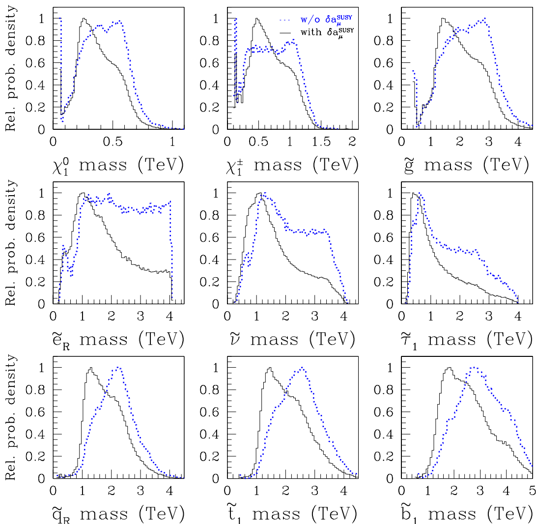
Figure 17: As in figure 5. The black solid (blue dotted) line is for the analysis including (excluding) the measurement of the anomalous magnetic moment of the muon, eq. (3.7). Both cases assume the “4 TeV range” priors.
