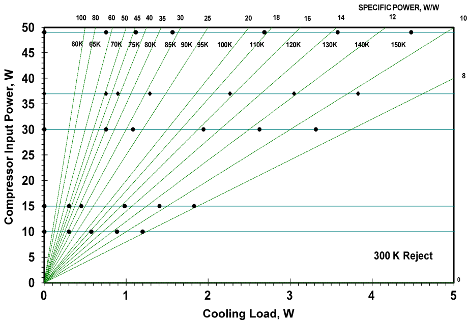
Figure 4. Microcooler performance map at 300K reject
