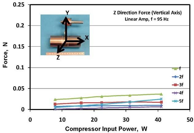
Figure 8. Microcooler exported vibration in Z axes without active vibration control
