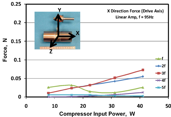
Figure 6. Microcooler exported vibration in X axes without active vibration control
