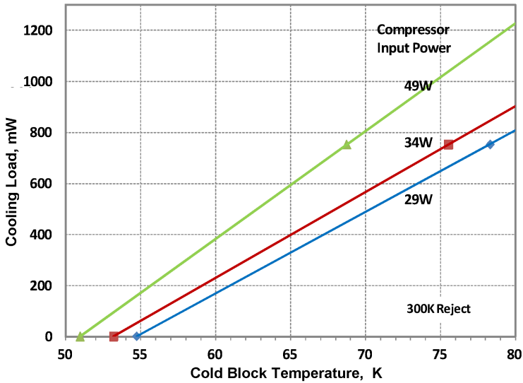
Figure 3. Microcooler load lines at 300K reject temperature
