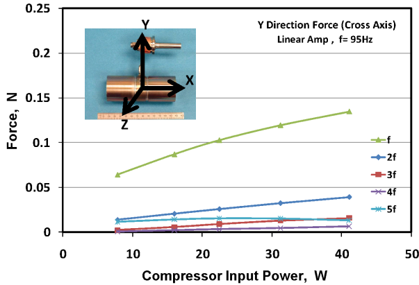
Figure 7. Microcooler exported vibration in Y axes without active vibration control
