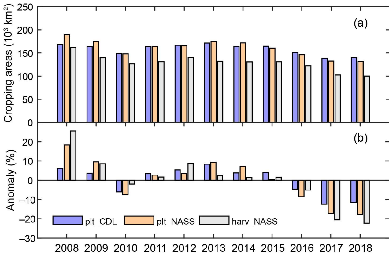
Figure 2. Interannual changes of winter wheat planted and harvested areas in the CONUS from 2008–2018 (plt_CD, plt_NASS, harv_NASS): (a) planted area and harvested area; (b) anomalies of planted area and harvested area for the multi-year averages from 2008–2018.
