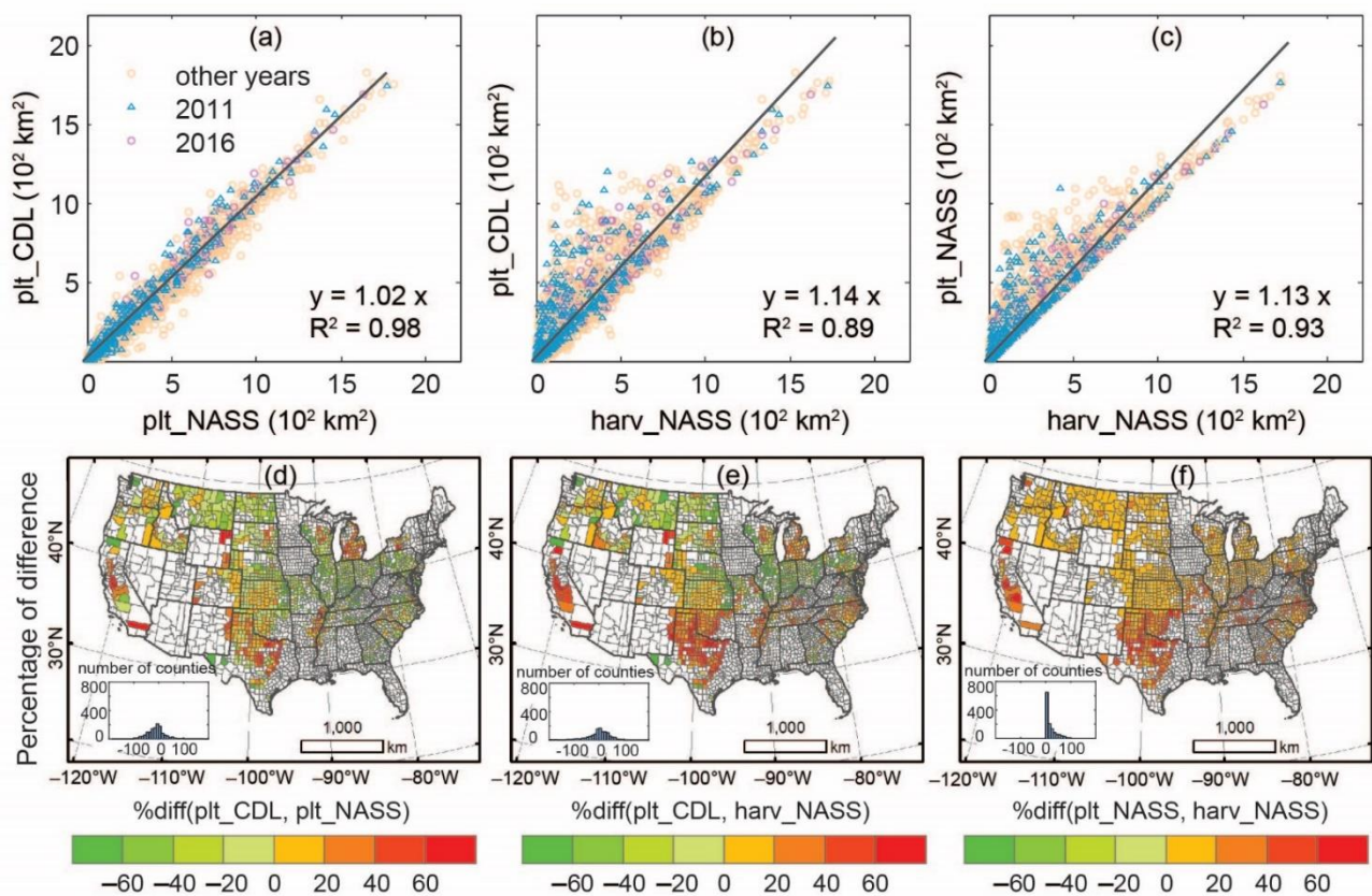
Figure 3. Comparisons between winter wheat planted areas and harvested area over CONUS from 2008–2018 at the county scale from the CDL and NASS datasets (plt_CD_L, plt_NASS, harv_NASS). (a) Planted area, (b,c) planted area vs. harvested area, (d–f) the spatial discrepancy (relative difference, %) in 2010 for planted area (d), and between planted area and harvested area (e,f). Year 2011 is a typical drought year over the winter wheat belt, and 2016 is a wet year.
