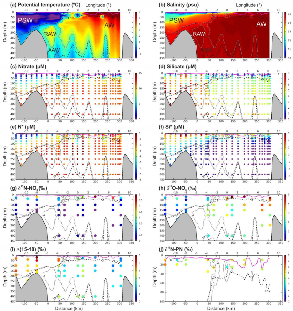
Figure 3. Sections of the upper 450m across the Fram Strait from cruise PS100 during July-August 2016. (a) Temperature, (b) Salinity, (c) Nitrate ( \mu\text{M} ), (d) Silicate ( \mu\text{M} ), (e) \text{N}^* ( \mu\text{M} ), (f) \text{Si}^* ( \mu\text{M} ), (g) \delta^{15}\text{N-NO}_3 (‰ vs. AIR), (h) \delta^{18}\text{O-NO}_3 (‰ vs. VSMOW), (i) \Delta(15-18) (‰), and (j) \delta^{15}\text{N-PN} (‰ vs. AIR). Contours and labelling as per Figure 2.
