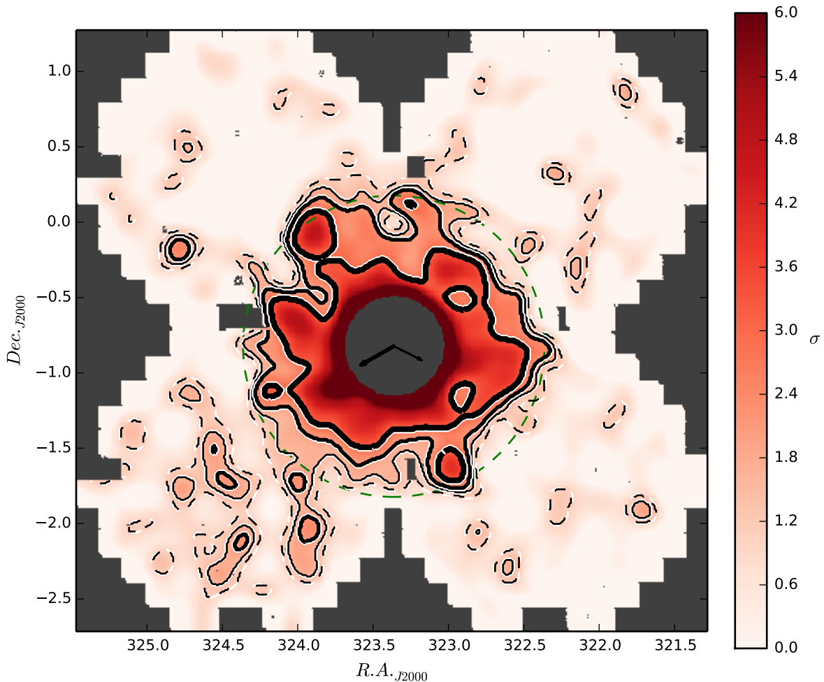
Figure 10. Stellar density distribution for the DECAM catalogue split into 36'' \times 36'' bins and smoothed using a gaussian kernel of width 4.8' . As for Figure 9 the colour scale represents the number of standard deviations above the mean background value that a given bin sits. The dashed contours indicate a level corresponding to 1\sigma above the mean bin density. Contours representing the 1.5\sigma , 2\sigma and 3\sigma levels are shown by solid lines, increasing in thickness. A circular region of radius 20' , almost twice the size of the nominal tidal radius, has been masked at the cluster centre. The outer dashed ring indicates a radius of 60' . The arrows are the same as Figure 9.
