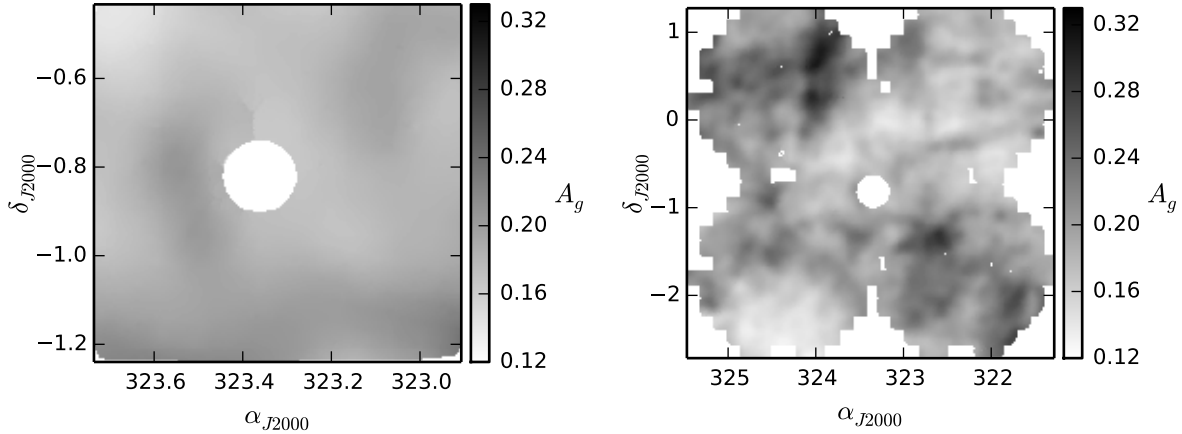
Figure 3. The A_g extinction map for sources appearing in SDSS DR12 (Ahn et al. 2014), based on the reddening maps of Schlegel et al. (1998), and smoothed with a gaussian function of width 36' . The MegaCam field of view is on the left, and DECam on the right. The excised inner cluster regions are the same as in Figure 1.
