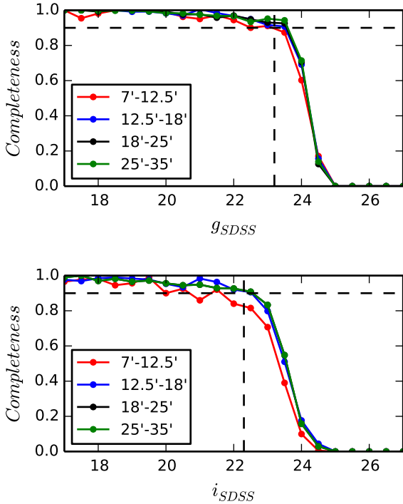
Figure 5. DECam completeness as a function of distance: g -band completeness is displayed in the top panel and i -band in the bottom panel. The vertical and horizontal dashed lines indicate the 90% completeness level and the corresponding magnitude adopted.
