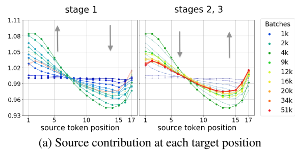
Figure 20: Changes in training: contribution of source token at each position to the whole target. Each line corresponds to a model state. The arrows show the direction of change when the training progresses. In the figures, all stages are shown, but the stages of interest are highlighted more prominently.
