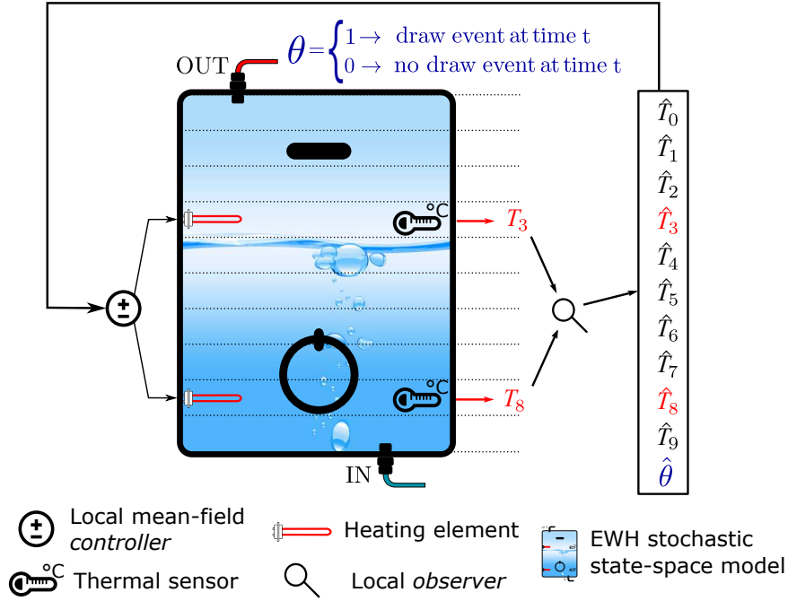
Figure 4: Schematic of the local controller of an EWH.
