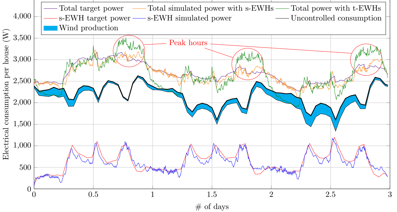
Figure 7: Simulation results with smartDESC controlled EWHs (s-EWHs) as opposed to traditional thermostatically controlled EWHs (t-EWHs) in a more complex scenario with forecasts on wind production; peak hours are circled in red.
