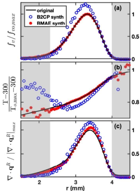
Figure 3: Profiles at z=10.8\text{mm} of: (a) soot volume fraction; (b) temperature; (c) radiative balance. The quantities are scaled by their peak values within the original fields shown in Fig.1 ( f_{vo,max}=15.7\text{ppm} , T_{o,max}=1961\text{K} , |\nabla \cdot \mathbf{q}_o^R|_{max}=39.5\text{kW}\cdot\text{m}^{-3} ). The white stripe represents the region producing 95% of the radiative power attributed to soot.
