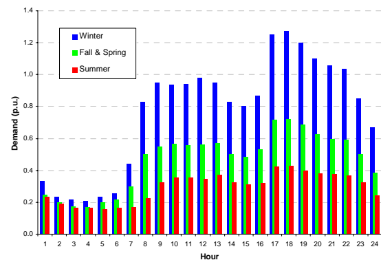
Fig. 2. Seasonal daily load profiles.
