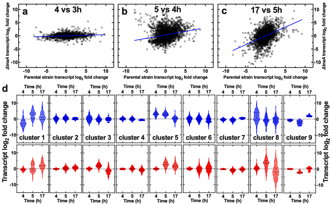
FIG 3 Genetic analysis of the consequences of the lack of tryptophanase. (a to c) Correlations between the log 2 fold changes in transcript reads for the parental and ΔtnaA strains between 4 and 3 h (a), 5 and 4 h (b), and 17 and 5 h (c). Each dot is the log 2 fold change in transcript reads for a single gene, and blue lines are linear regressions to the data returning Pearson correlation coefficient R values of 0.15, 0.23, and 0.43, respectively. Transcript reads were measured via RNA sequencing of samples in biological triplicates and are reported in Data Set S1. (d) Cluster analysis of the above-described transcriptomic data returned nine clusters with distinct patterns of gene regulation for the parental and ΔtnaA strains (top and bottom rows, respectively). Each dot represents the log 2 fold change in transcript reads for a single gene, dashed lines indicate the median and quartiles of each distribution, and dotted lines indicate a log 2 fold change of zero. The lists of genes belonging to each cluster are reported in Data Set S1.
