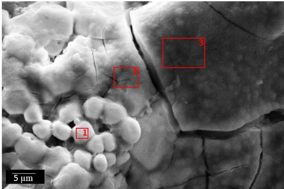
Figure 108. SEM image of top surface of CBR 1-12. Area 1 contains CeO 2 particles covered by melt-like phase. Area 2 contains melt-like structure and cracks. Area 3 contains melt-like structure and cracks, but area 3 is closer to a crack than area 2.
