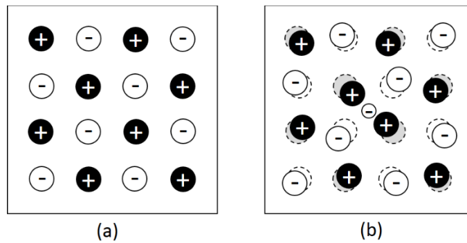
Figure 96. Schematic diagram of (a) a perfect ionic structure and (b) an ionic structure with an electron defect which attracts the positive and repulses the negative ions causing hopping motions (modified from [184]).
