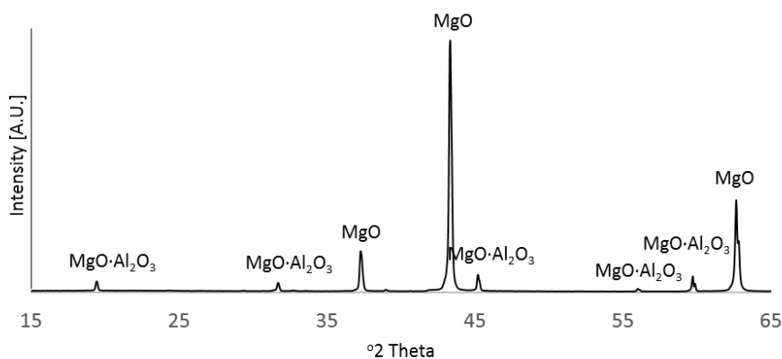
Figure 59. XRD of refractory brick.
