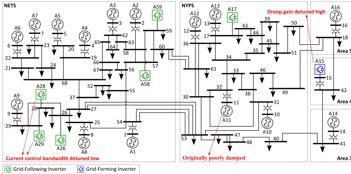
Fig. 4. Modified NETS-NYPS 68 bus system, with 6 extra grid-following inverters, and a grid-forming inverter replacing the synchronous machine at bus 15.
