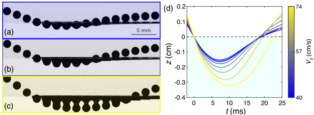
Figure 2: Rebound data for superhydrophobic spheres with radius R_s = 0.083 cm and density \rho_s = 2.2 g/cm 3 . (a-c) Sequence of images with different impact speeds V_0 : (a) 40.2 \pm 0.7 cm/s, (b) 53.7 \pm 0.7 cm/s, (c) 73.6 \pm 0.6 cm/s. Images are evenly spaced in time by 2 ms, corresponding to 20 frames. (d) Trajectories of the bottom of the spheres (relative to the undisturbed free surface height) measured for 8 different impact velocities. Shown are the average trajectories over all trials at a fixed release height with outliers removed, as described in the text. Videos corresponding to the trials shown in (a)-(c) are available as supplementary material.
