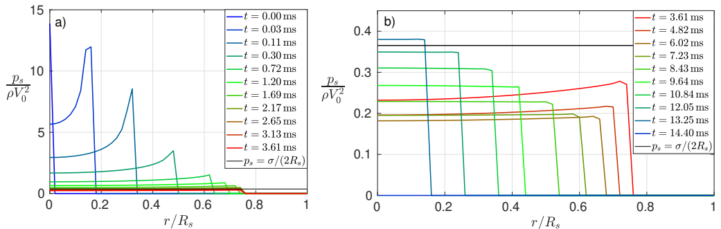
Figure 8: Evolution of pressure distribution as predicted by the linearised model. Panel (a) shows the pressure distributions as the pressed area expands following impact, and panel (b) shows the pressure distribution as the pressed area contracts before lift-off ( R_s = 0.83 mm, \rho_s = 1.2 g/cm 3 , V_0 = 34.45 cm/s). The black horizontal line indicates the contribution of surface tension to the pressure distribution and thus serves as a reference level.
