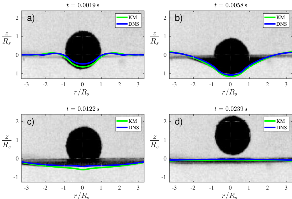
Figure 7: Surface profile predictions superimposed onto experimental high speed camera images for R_s = 0.83 mm, \rho_s = 1.2 gr/cm 3 and V_0 = 34.45 cm/s.
