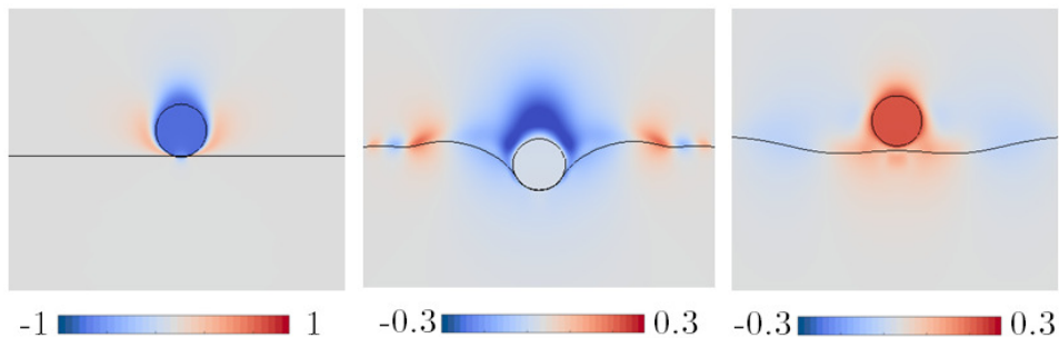
Figure 4: Typical bouncing behaviour as observed in the direct numerical simulations for a case described by sphere radius R_s = 0.083 cm, density \rho_s = 2.2 g/cm 3 and impact speed V_0 = 56.67 cm/s. The background colour represents the dimensionless vertical velocity field, with the relevant interfaces also highlighted in black. The three illustrated instances represent, in dimensionless time units: (left) t \approx 1.0 , as the impactor touches the surface, (middle) t \approx 4.5 , as the impactor reaches its maximum depth and (right) t \approx 10.0 , as the impactor leaves the surface for its first bounce.
