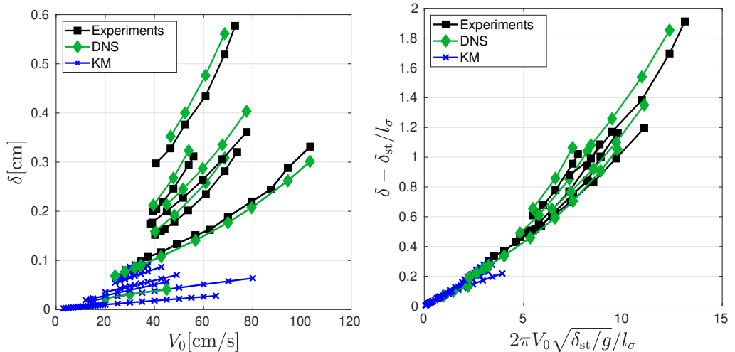
Figure 14: Collapse of the maximum surface deflection on the basis of the non-linear spring model at the equilibrium deflection. Left panel: the full set of experimental and simulated data for which the sphere returns to the impact height. Right panel: the same data re-scaled using the variable suggested by the boundary layer analysis. The vertical axis on the right panel is normalised using the capillary length, l_\sigma = \sqrt{\sigma/\rho g} .
