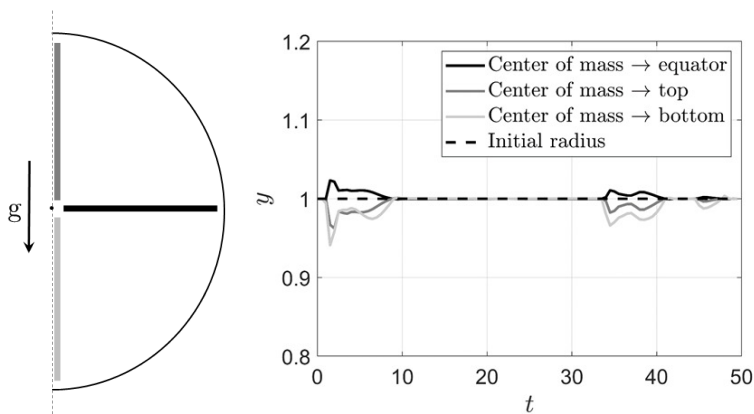
Figure 5: Pseudo-solid deformation study for a representative test case described by an impacting sphere of radius R_s = 0.83 mm, \rho_s = 2.2 g/cm 3 and V_0 = 56.67 cm/s. (Left) Sketch of measured segments as distances from the centre of mass of the impactor to its relevant extremities. (Right) Segment size evolution as a function of dimensionless time, compared to a reference undeformed y = 1 radius, indicated here with a dashed line.
