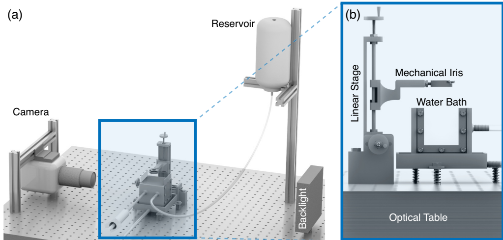
Figure 1: (a) Rendering of the complete experimental setup, including the high-speed camera, water bath, linear stages, water reservoir, and backlight. (b) Closer view of the water bath and linear-stage system, viewed from the perspective of the camera.
