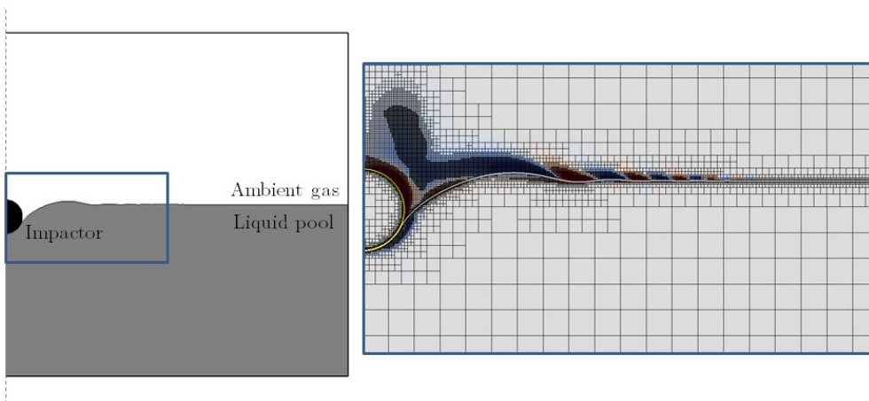
Figure 3: Axisymmetric simulation domain of size 20R_s \times 20R_s , with R_s denoting the impactor radius. The inset illustrates the adaptive mesh refinement strategy, with changes in vorticity (shown as background colour) and interfacial locations used as primary criteria. A video corresponding to this particular case (expanded on in Figures 4-5 as well) is available as supplementary material.
