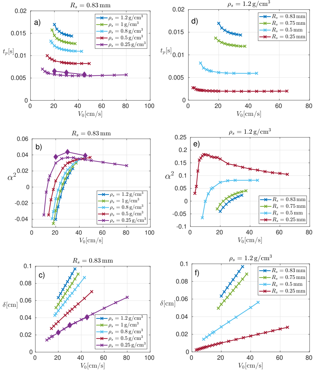
Figure 12: Rebound metrics for weak impacts. Cross (+) markers correspond to KM predictions and diamond (◆) markers to DNS predictions. In these impacts, different rebound metrics were used. These are the pressing time t_p , defined as the length of the time interval over which the south pole of the sphere is in direct contact with the fluid surface; and the coefficient of restitution squared \alpha^2 , which can take negative values when the total energy transfer during the rebound is greater than the kinetic energy of the sphere as it starts its contact with the bath. All relevant notation and parameter values are provided in Table 1.
