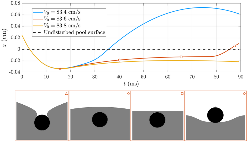
Figure 11: “Resurrection” phenomenon observed using DNS for a pseudo-solid with radius R_s = 0.124 cm and density \rho_s = 1.2 g/cm 3 , impacting with velocity V_0 = 83.6 cm/s. Small impact velocity variations (of \pm 0.2 cm/s) result in either bouncing or sinking. Lines in the top panel represent the z -position of the centre of mass of the pseudo-solid as a function of time in each of these cases, while symbols indicate representative time steps in the flow evolution for the “resurrection” dynamics (illustrated in the bottom panel). A video summary contrasting these three scenarios is available as supplementary material.
