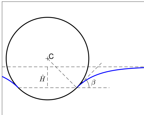
Figure 13: Schematic diagram for the quasi-static analysis. Point C corresponds to the centre of the sphere, \hat{H} is the depth of the boundary of the contact line, and \beta is the angle formed between the horizontal and the free surface, where it meets the solid.
