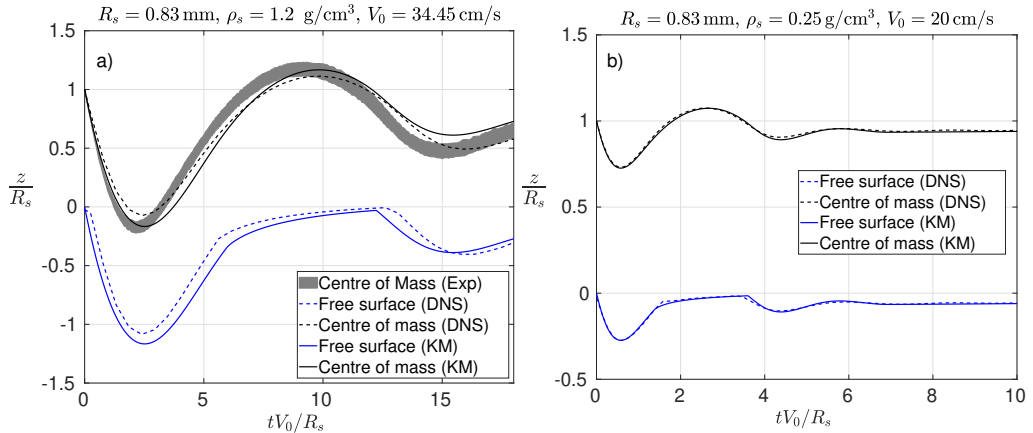
Figure 6: Comparison of predicted and measured trajectories. Panel (a) shows the resulting trajectory of the centre of mass in experiments (Exp) versus those obtained via direct numerical simulation (DNS) and kinematic match (KM) calculations. The width of the shaded regions that describe the experimental results enclose one standard deviation above and below the mean experimental trajectory. Panel (b) compares the results of the two numerical methods in the low Weber number regime, which is not accessible in the present experiments. Both panels also include the free-surface elevation at the centre of the bath, i.e. directly below the south pole of the sphere (the impact point), as obtained from DNS and KM simulations. Videos of the KM simulation for the case in panel (a) are available as supplementary material.
