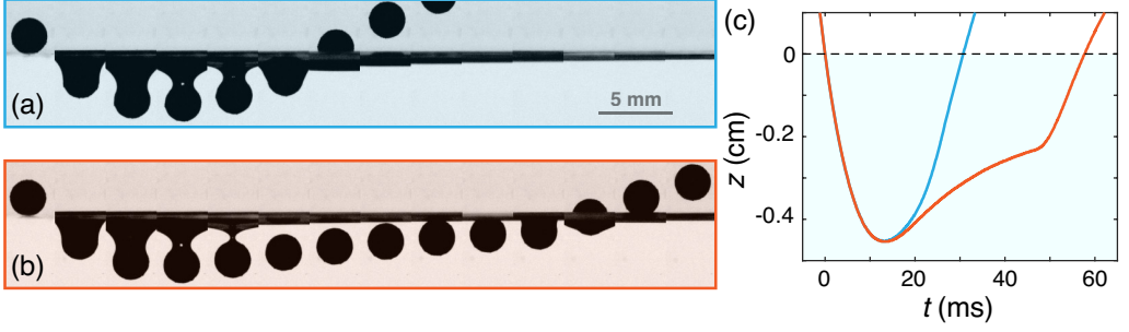
Figure 10: Two behaviours observed in experiment for nearly identical impact velocities for identical spheres with radius R_s = 0.124 cm and density \rho_s = 1.2 g/cm 3 , just before sinking threshold. (a) Standard rebound, V_0 = 86.7 \pm 1.7 cm/s. (b) “Resurrection” phenomenon where cavity pinches off yet the sphere eventually resurfaces and rebounds completely, V_0 = 87.4 \pm 3.5 cm/s. Images are evenly spaced in time by 4.8 ms, corresponding to 48 frames. (c) Trajectories associated with the images shown in parts (a) and (b). Videos corresponding to the trials shown in (a) and (b) are available as supplementary material.
