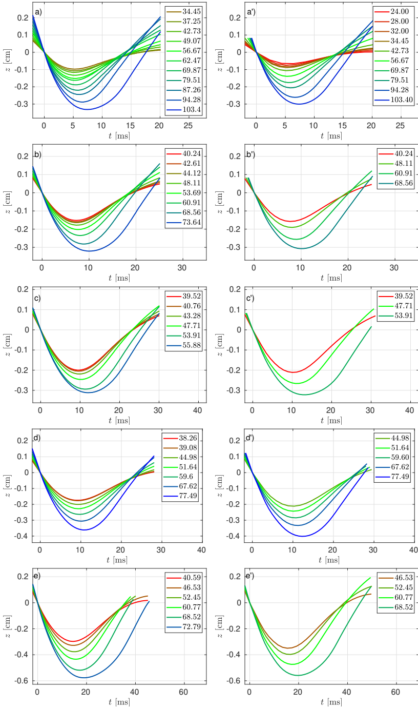
Figure 16: Average south pole trajectories for each sphere in experiments (a-e) and DNS south pole trajectories for the corresponding pseudo-spheres (a'-e'). Trajectories are colour coded by impact speed as indicated in the legends (in cm/s). (a-a') \rho_s = 1.2 \text{ g/cm}^3 , R_s = 0.83 \text{ mm} , (b-b') \rho_s = 2.2 \text{ g/cm}^3 , R_s = 0.83 \text{ mm} , (c-c') \rho_s = 3.2 \text{ g/cm}^3 , R_s = 0.83 \text{ mm} , (d-d') \rho_s = 1.2 \text{ g/cm}^3 , R_s = 1.24 \text{ mm} , (e-e') \rho_s = 1.2 \text{ g/cm}^3 , R_s = 1.64 \text{ mm} .
