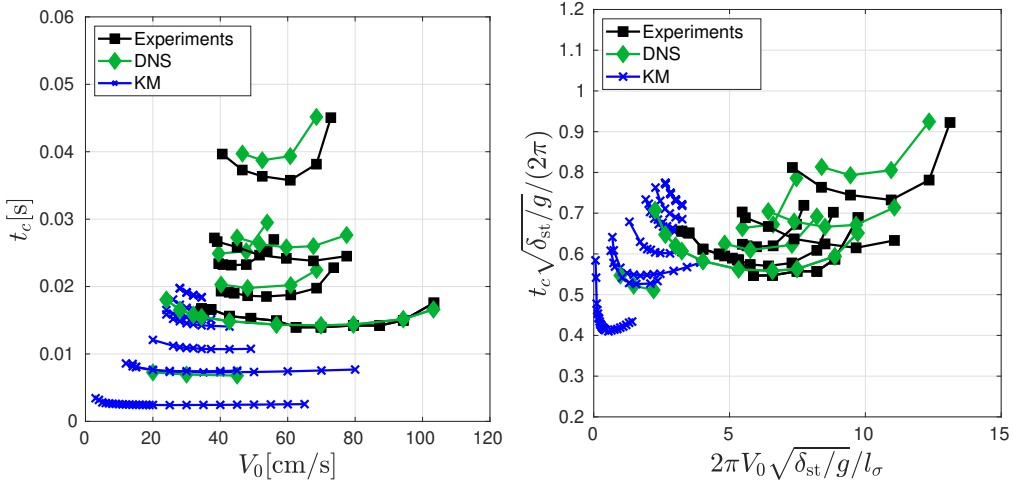
Figure 15: Collapse of the contact time on the basis of the period of oscillation of the spring model. Left panel shows the full set of experimental and simulated data for which the sphere returns to the impact height. Right panel shows the same data re-scaled using the variables suggested by the boundary layer analysis.
