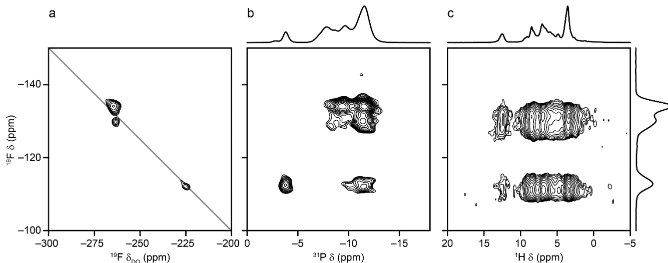
Figure 4. (a) ^{19}\text{F} (14.1 T, 55 kHz DQMAS), (b) ^{19}\text{F} - ^{31}\text{P} (14.1 T, 50 kHz MAS) CP-HETCOR and (c) ^{19}\text{F} - ^1\text{H} (9.4 T, 40 kHz MAS) HMQC spectra of GaPO-34[mimH]. Note that, for presentation purposes, the spectrum in (a) has been rotated such that \delta_2 (the ^{19}\text{F} MAS dimension) is along the vertical axis. The grey line in (a) shows the \delta_1 = 2 \delta_2 double-quantum autocorrelation diagonal. The ^1\text{H} , ^{19}\text{F} and ^{31}\text{P} NMR spectra from Figure 3 are shown along the relevant axes. See Supporting Information (S1) for further experimental details.
