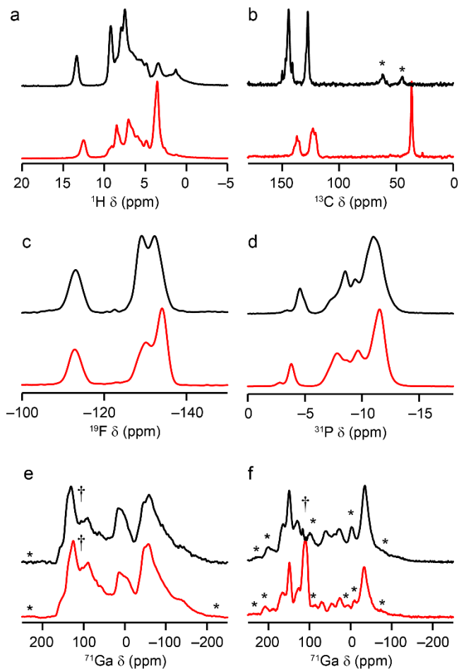
Figure 3. Solid-state NMR spectra of GaPO-34A[pyH] (black): (a) ^1\text{H} (14.1 T 55 kHz MAS), (b) ^{13}\text{C} (CP 14.1 T 12.5 kHz MAS), (c) ^{19}\text{F} (14.1 T 55 kHz MAS), (d) ^{31}\text{P} (CP 14.1 T 14 kHz MAS 293 K), (e) ^{71}\text{Ga} (20 T 50 kHz MAS) and (f) ^{71}\text{Ga} (34.1 T, 18 kHz MAS) and GaPO-34A[mimH] (red): (a) ^1\text{H} (14.1 T 60 kHz MAS), (b) ^{13}\text{C} (CP 14.1 T 12.5 kHz MAS), (c) ^{19}\text{F} (14.1 T 55 kHz MAS), (d) ^{31}\text{P} (CP 14.1 T 14 kHz MAS, 293 K), (e) ^{71}\text{Ga} (20 T 60 kHz MAS) and (f) ^{71}\text{Ga} (34.6 T, 18 kHz MAS). Asterisks (*) indicate spinning sidebands and daggers (†) indicate the position of the ^{71}\text{Ga} signal from GaPO 4 berlinite (~5% impurity in both samples). See Supporting Information (S1) for further experimental details.
