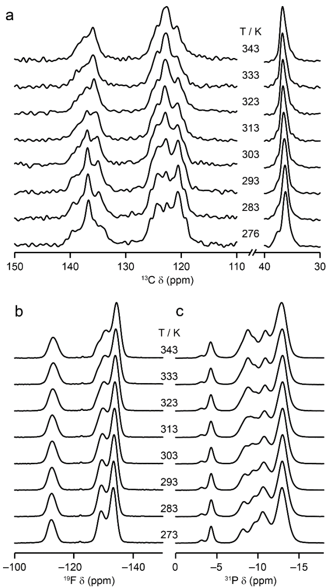
Figure 9. (a) ^{13}\text{C} (9.4 T, 12.5 kHz CP MAS), (b) ^{19}\text{F} (14.1 T, 35 kHz MAS) and (c) ^{31}\text{P} (14.1 T, 12.5 kHz CP MAS) variable-temperature NMR spectra of GaPO-34[mimH]. See Supporting Information (S1) for further experimental details.
