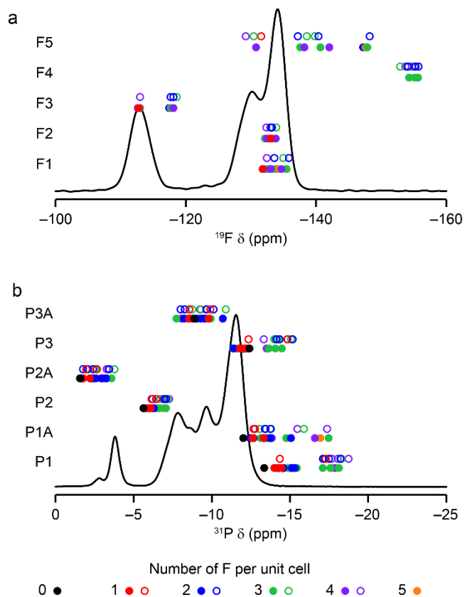
Figure 7. (a) ^{19}\text{F} and (b) ^{31}\text{P} \delta_{\text{iso}} calculated for the different sites in models of GaPO-34A[mimH] with 0-5 F anions per unit cell (and all other anion sites occupied by OH). Calculated points are overlaid onto the experimental spectra presented in Figure 3. Open points indicate structures with an unfavorable E_{\text{mix}} and filled points indicate a favorable E_{\text{mix}} (note that, for the end members with 0 and 5 F per cell, there is only one model with E_{\text{mix}} = 0 ). See Supporting Information (S3) for further details and models with different SDA orientations.
