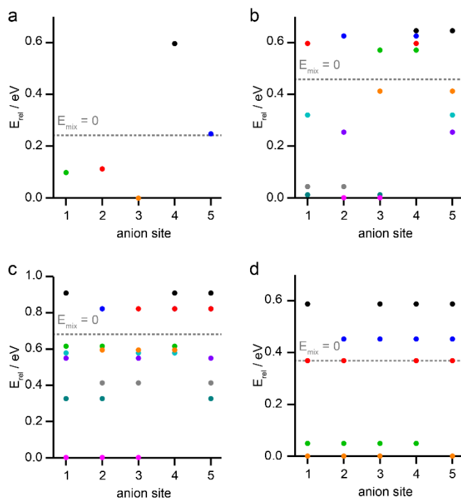
Figure 5. Plots of relative energies ( E_{\text{rel}} ) of models of GaPO-34A[mimH] with different numbers of anion sites occupied by F and all remaining anion sites occupied by OH. Models have (a) one, (b) two, (c) three and (d) four F anions per unit cell. Dashed lines indicate E_{\text{mix}} = 0 for each specified composition. See Supporting Information (S3) for further details and additional models with different SDA orientations.
