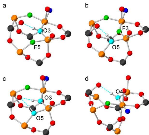
Figure 6. Hydrogen bonding arrangements for OH located on anion sites 3 and 5 in optimized models of GaPO-34A[mimH], where all other anion sites are occupied by F and the SDA is in orientation A. (a) OH on site 3, F on site 5 – the OH...O distance is 1.65 Å and the O-H...O angle is 166.6°, (b) F on site 3, OH on site 5 – the OH...O distance is 1.94 Å and the O-H...O angle is 172.0°, (c) OH on sites 3 and 5 – for site 3 the OH...O distance is 1.74 Å and the O-H...O angle is 158.5° and for site 5 the OH...O distance is 2.08 Å and the O-H...O angle is 158.6°. (d) Hydrogen bonding arrangement for OH in anion site 4 with all other anion sites occupied by F and the SDA in the A orientation – the OH...O distance is 1.90 Å and the O-H...O angle is 175.1°. Atoms are colored with H = light grey, framework O = red, hydroxyl O = cyan, water O = dark blue, F = green, P = dark grey and Ga = orange.
