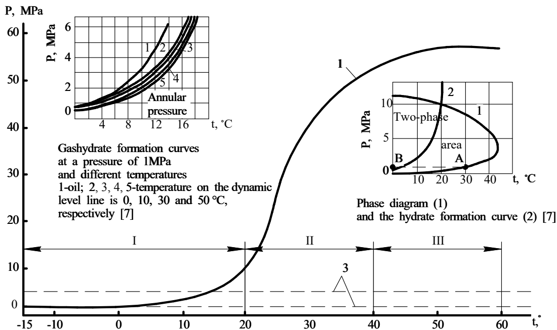
Fig. 3. Graphs of the hydrate formation curve (1) in the annulus of the oil well: zone I – maximum probability of hydrate formation (90–100 %); zone II – average probability of hydrate formation (40–50 %); zone III – minimum probability of hydrate formation (10–20 %); 3 – lines of pressure-temperature conditions
