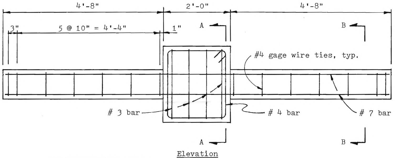
Figure 1. Column reinforcing bar design.
