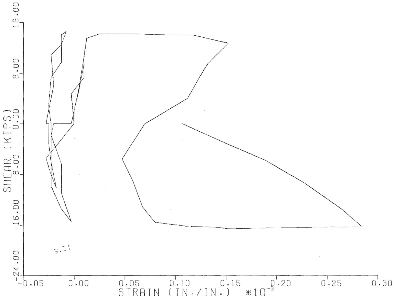
Figure 3.21 Specimen 2, strain on packaging band next to joint for deflection cycles 1, 4, and 7.
