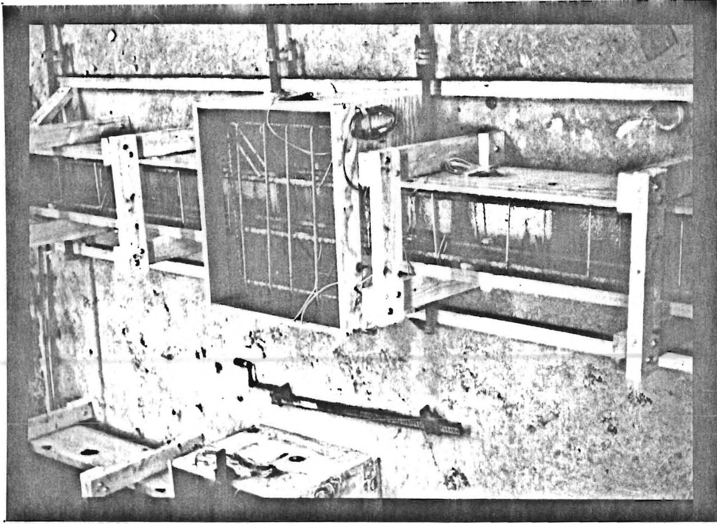
Figure 2. Reinforcing bar cage in column forms.
