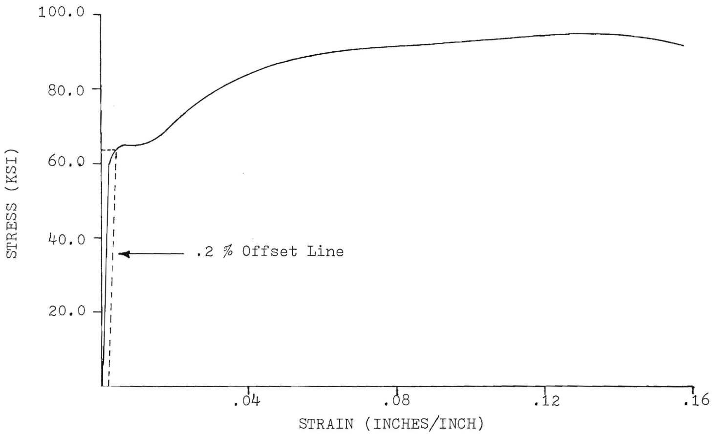
Figure A.3 - Average Stress-Strain Curve for No. 4 Reinforcing Steel Bar
