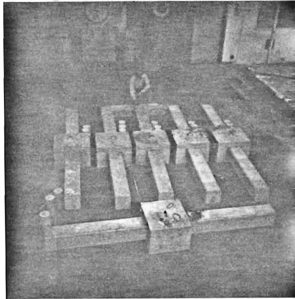
Figure 4. Six model columns ready for strengthening procedures
