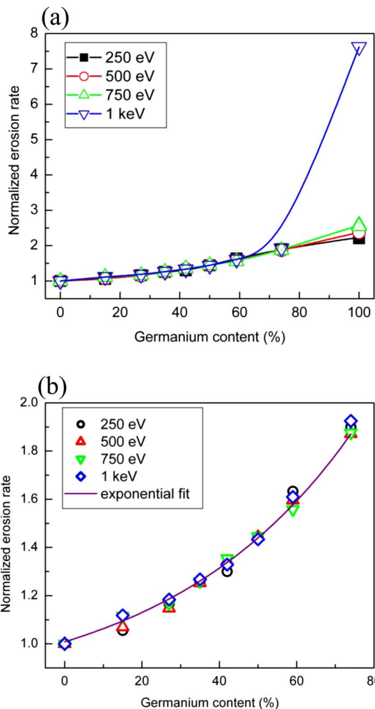
FIG. 6. (Color online) (a) Normalized erosion rates as a function of germanium content for different primary beam energies. (b) Normalized silicon Si 1-x Ge x erosion rates and exponential fit as a function of germanium content.
