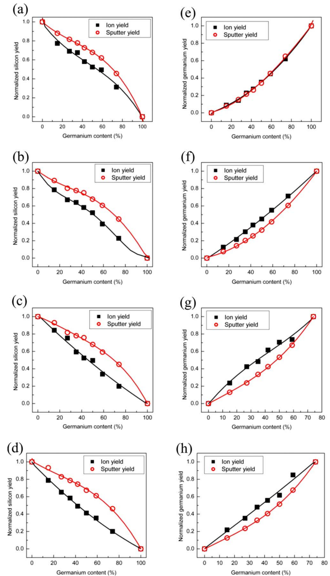
FIG. 8. (Color online) Normalized silicon and germanium ion and sputter yields as a function of germanium content. (a) 250 eV silicon, (b) 500 eV silicon, (c) 750 eV silicon (d) 1 keV silicon, (e) 250 eV germanium, (f) 500 eV germanium, (g) 750 eV germanium, and (h) 1 keV germanium.
