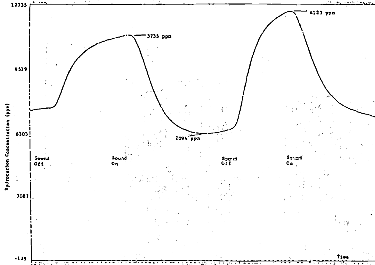
Figure 25: The Variation of Hydrocarbon Concentration with Time in Test No. 20
