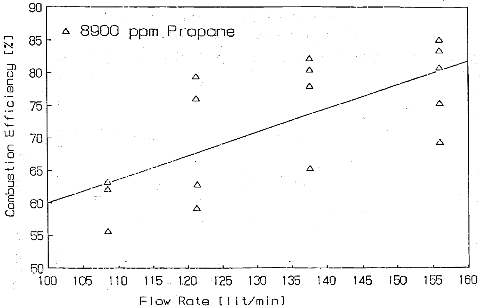
Figure 13: Dependence of Combustion Efficiency on Flow Rate of Propane/Air mixture at Propane Concentrations of 8900 ppm.
