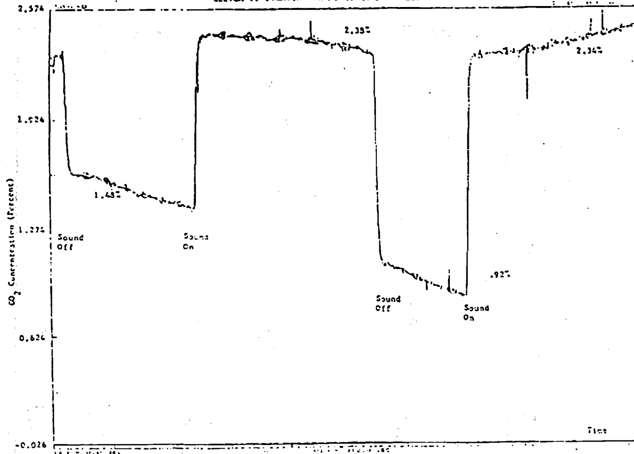
Figure 26: The Variation of CO_2 Concentration with Time in Test No. 30
