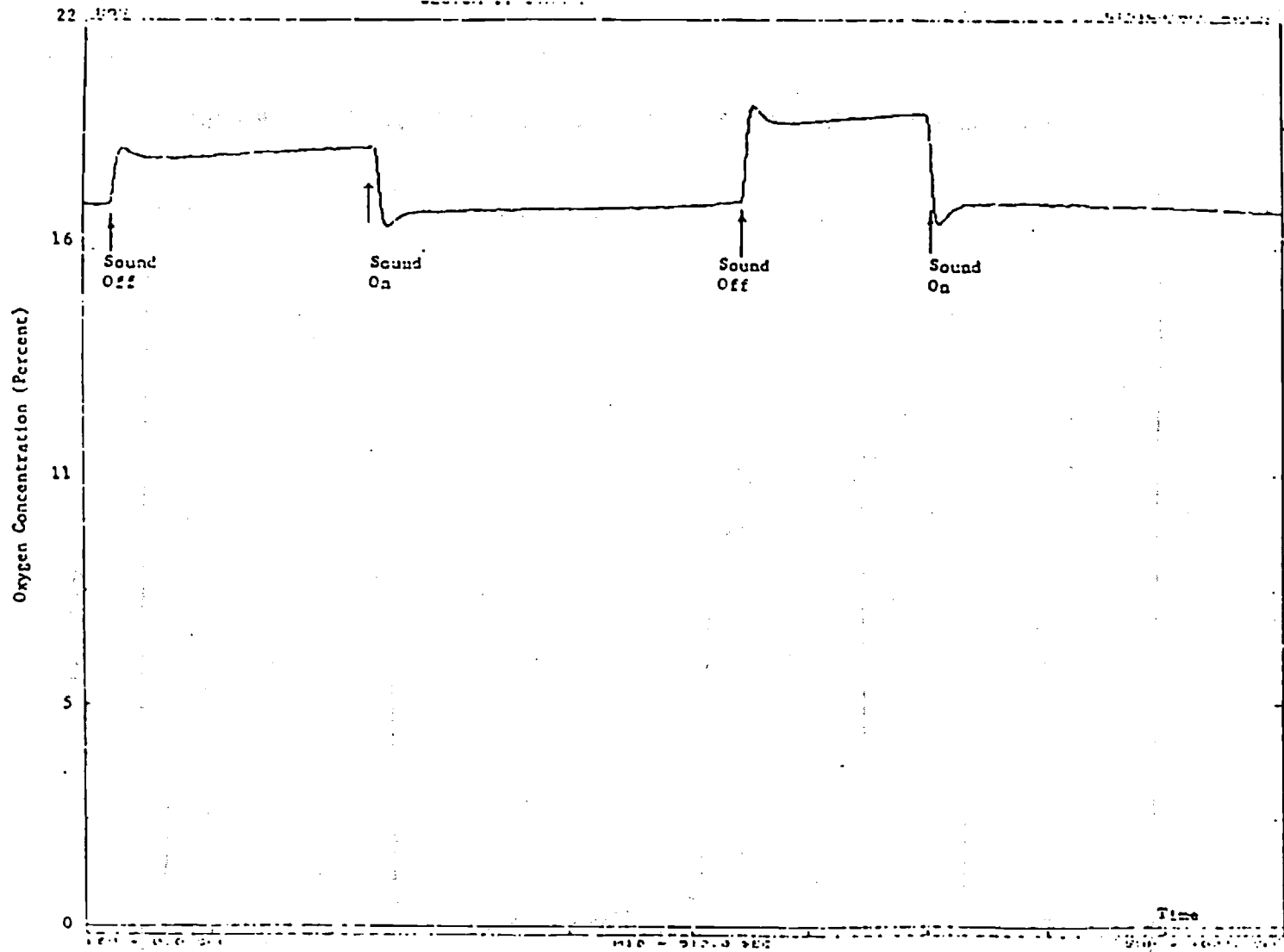
Figure 27: The Variation of Oxygen Concentration with Time in Test No. 30
