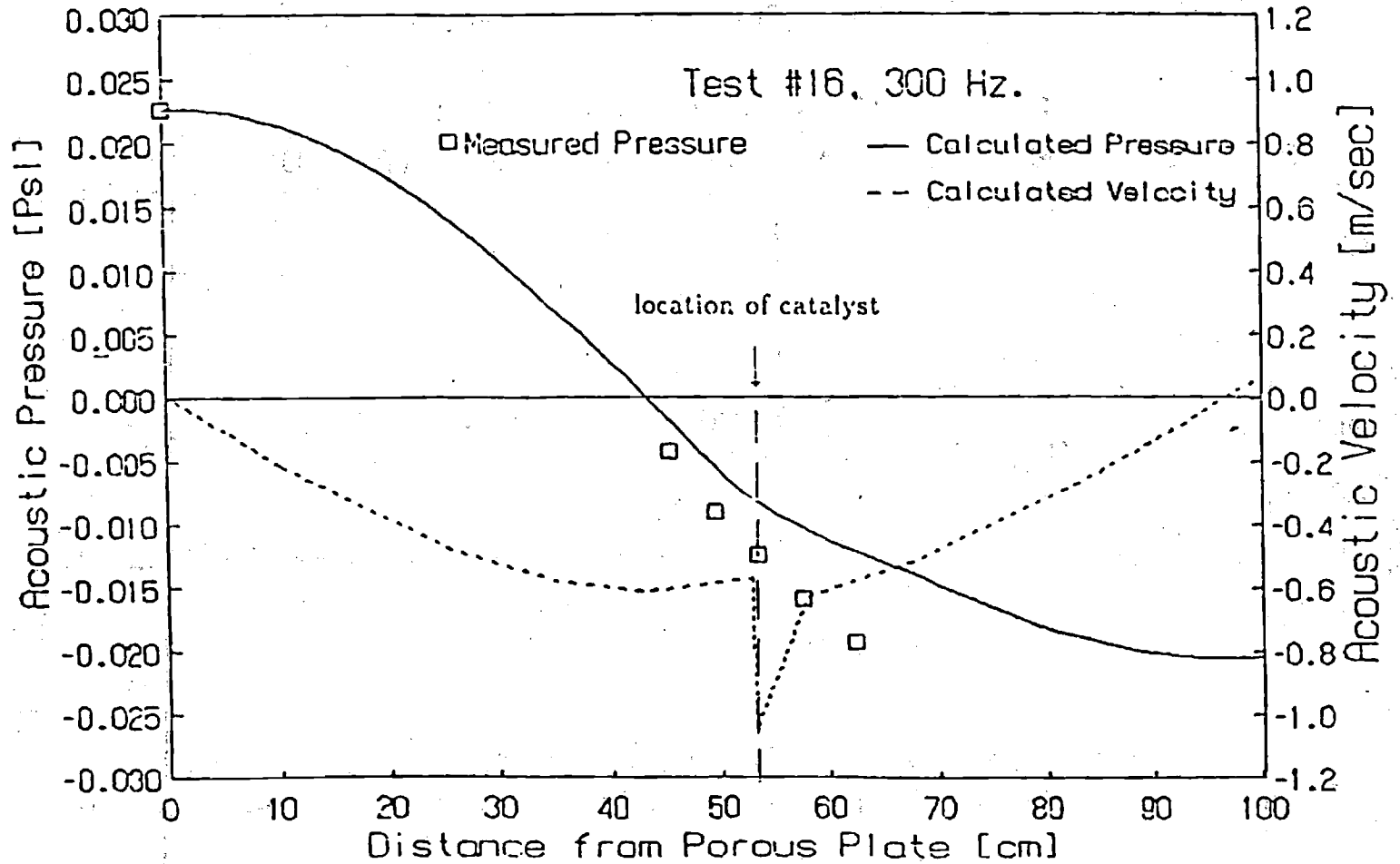
Figure 7: Comparison of Measured and Calculated Acoustic Pressure and Velocity for a Frequency of 300 Hz in Test No. 16
