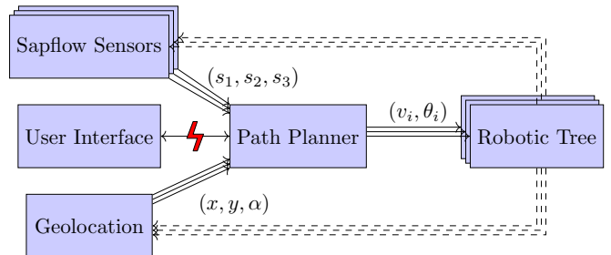
Fig. 6: Software architecture: Each tree has three sap flow sensor that are used as inputs for the Path Planner. The Path Planner also retrieves the current position and orientation of each robot from the geolocation system, and then computes the traction speed and orientation of each wheel of each AGV. Users may also give direct orders to the Path Planner when necessary. The variables (s_1, s_2, s_3) , (x, y, \alpha) and (v_i, \theta_i) are developed in Section IV.
