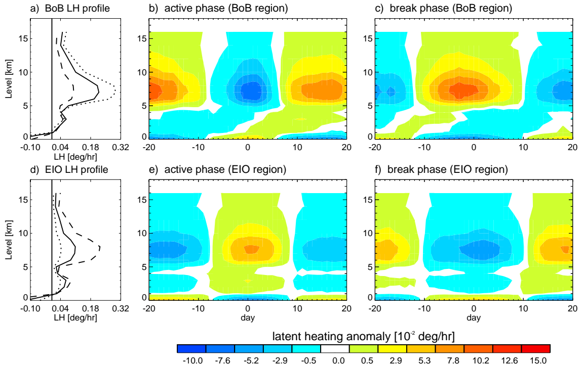
Figure 9: Same as Fig. 6 but using the TRMM-2A12 dataset.
