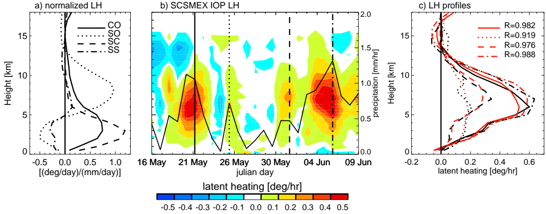
Figure 11: LH profiles basis for the CSH algorithm (i.e., look-up tables) for ocean convective (CO), ocean stratiform (SO), shallow convective (SC) and shallow stratiform (SS) precipitating systems. Profiles are normalized by rainfall rate [(deg/day)/(mm/day)]. (b) Evolution of LH vertical profiles [deg/hr] from the SCSMEX NESA dataset from May 16 to June 9, 1998 over the SCS region. Yellow-red shading is proportional to positive LH values. (c) LH profiles estimated for the 4 days (05/21/08, 05/25/08, 06/01/08 and 06/06/08) represented by vertical lines in Fig. 11b using the SCSMEX dataset (black lines) and computed using multi-linear regression (red lines) from the normalized profiles in Fig. 11a (see text for more details).
