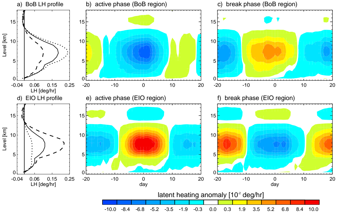
Figure 6: Mean summer LH profiles (black solid line) and mean profiles for the active (dashed line) and break periods (dotted line) of the MISO (left panels) over the BoB and EIO regions. Time evolution composites of summer LH [deg/hr] anomalies (time-height diagrams) \pm 20 days of the day 0 active/break conditions defined in the text (right panels). The TRMM-CSH daily dataset for 1998-2006 summer seasons was used. Top panels correspond to the BoB region and bottom panels to the EIO region.
