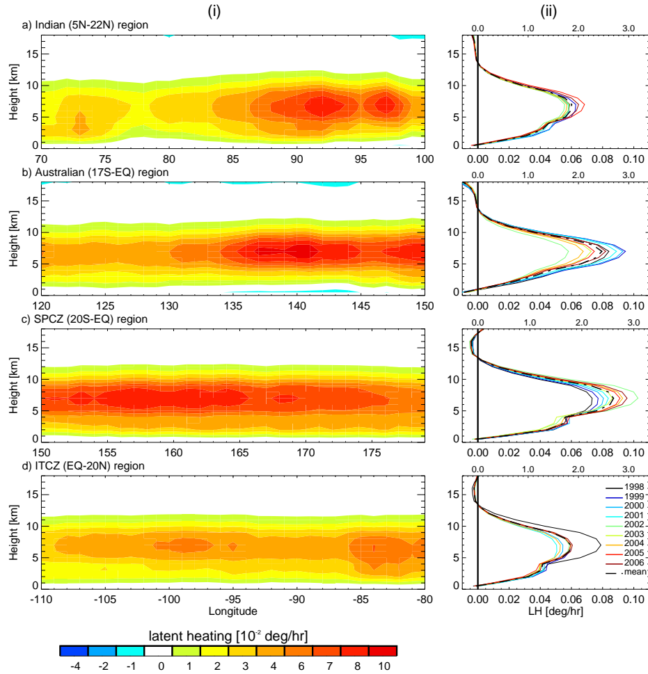
Figure 2: Longitude-height distributions (i panels) and the average vertical profile of LH [deg/hr] for each year of the 1998-2006 profiles (ii panels) for the (a) Indian ( 5^{\circ}\text{N} - 22^{\circ}\text{N} , 70^{\circ}\text{E} - 100^{\circ}\text{E} ) and (b) Australian ( 17^{\circ}\text{S} - 0^{\circ}\text{S} , 120^{\circ}\text{E} - 150^{\circ}\text{E} ) monsoon regions, (c) SPCZ ( 20^{\circ}\text{S} - 0^{\circ}\text{S} , 160^{\circ}\text{E} - 179^{\circ}\text{E} ) and (d) East Pacific ITCZ ( 0^{\circ}\text{N} - 20^{\circ}\text{N} , 125^{\circ}\text{W} - 80^{\circ}\text{W} ) regions using monthly TRMM-CSH retrievals. Average LH profiles are represented by the dashed lines and yearly profiles by the colored lines.
