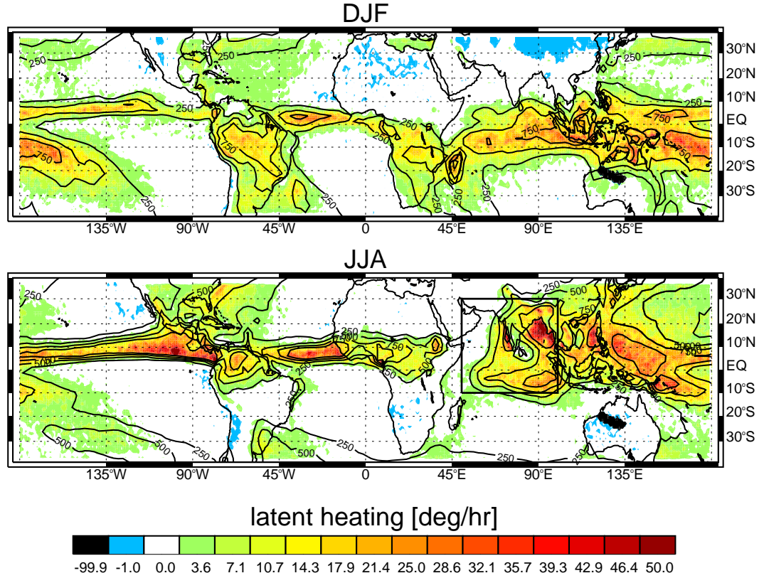
Figure 1: Vertically integrated LH distribution [deg/hr relative to color bar] for boreal (June-August) and austral (December-February) summers averaged over the 1998-2006 period using the monthly TRMM-CSH dataset. Black contours show mean seasonal precipitation [mm] using monthly GPCP data. The black box corresponds to the south-Asian monsoon region that is the focus of the study.
