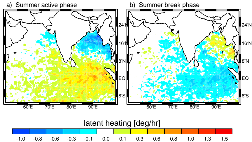
Figure 8: Same as Fig. 5 but using the TRMM-2A12 dataset.
