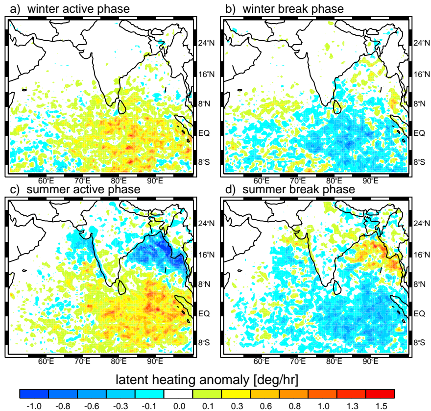
Figure 5: Composites of vertically integrated LH anomalies [deg/hr] for a) and c) active and b) and d) break phases of the intraseasonal oscillation of the SAMR for the extended winter season (November-March: NDJFM) and extended summer season (May-September: MJJAS), respectively. Color shading is relative to the scale at the bottom of the figure. The daily TRMM-CSH dataset for the 1998-2006 period was used in this figure.
