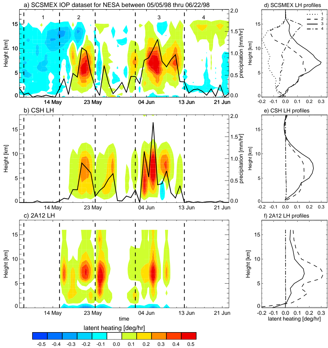
Figure 10: Evolution of LH vertical profiles [deg/hr] from (a) the SCSMEX campaign from Johnson and Ciesielski (2002, see text for details), (b) the TRMM-CSH and (c) the TRMM-2A12 datasets during May 5 to June 22, 1998 over the SCS region. Yellow-red shading is proportional to positive LH values. The solid black line in (a) corresponds to the time series of precipitation from the SCSMEX observational period and in (b) from the TRMM-3G68 PR based product. The right panels show averaged LH profiles for four periods denoted by the vertical dashed lines in Fig. 10a using each dataset as described in the text. The periods are from 05/07/98 to 05/14/98, 05/15/98 to 05/23/98, 06/01/98 to 05/12/98, and 06/01/98 to 05/12/98.
