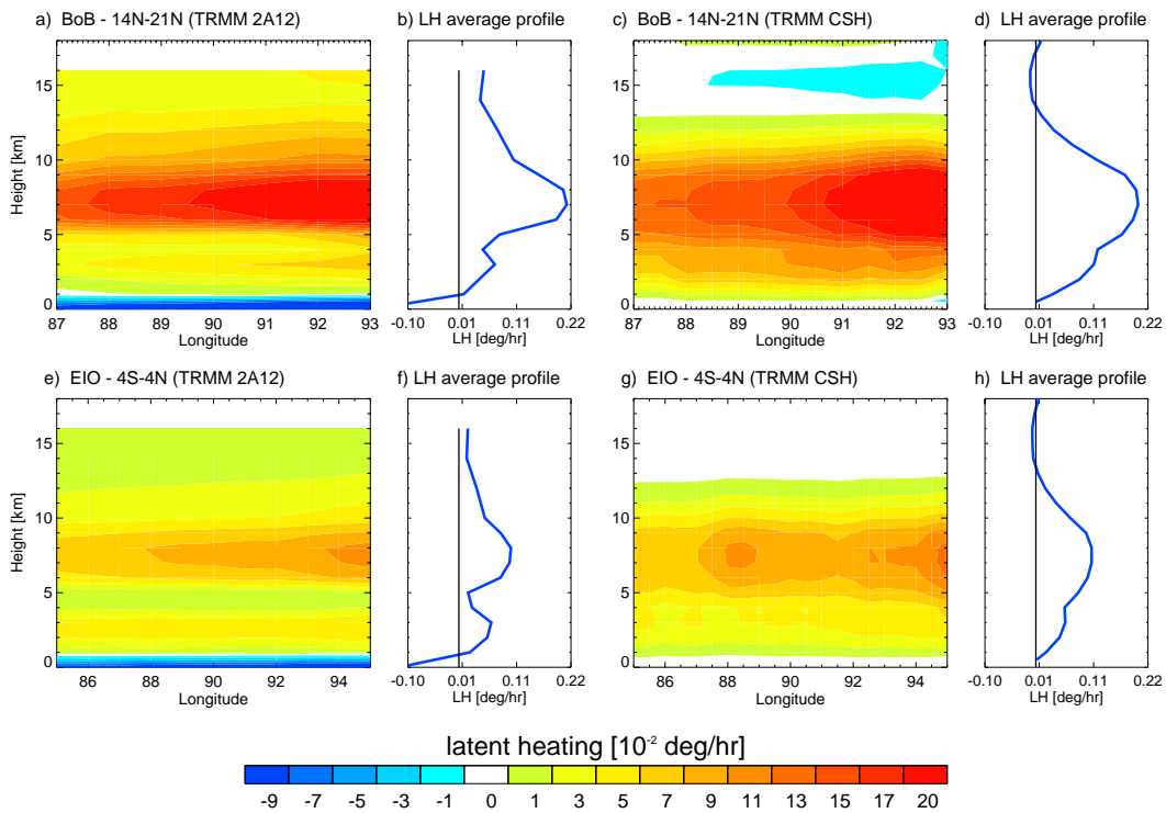
Figure 7: Vertical distribution of latitudinally averaged LH [deg/hr] for the BoB (top panels) and EIO (bottom panels) regions using both the TRMM-2A12 (left panels) and TRMM-CSH (right panels) datasets. Extended summer periods for the 1998-2006 period for both datasets were used. The mean LH vertical profile is shown next to each panel.
