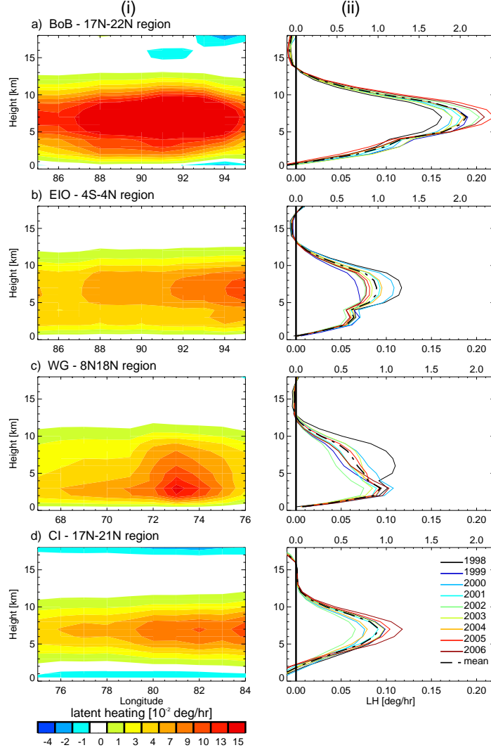
Figure 4: Same as Fig. 2 but for extended summer periods over (a) BoB, (b) EIO, (c) WG and (d) CI.
