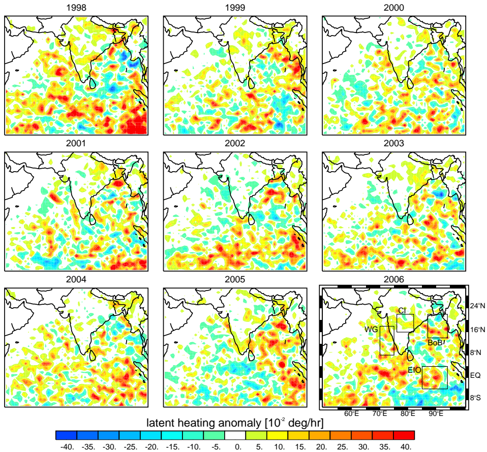
Figure 3: Vertically integrated LH anomalies [deg/hr] for each year between 1998 and 2006 for the SAMR using monthly TRMM-CSH data. Blue shading (yellow-red shading) corresponds to negative (positive) LH anomalies. The boxes in the lower right corner correspond to the regions considered in this study: Bay of Bengal (BoB), equatorial Indian Ocean (EIO), Western Ghats (WG) and central India (CI).
