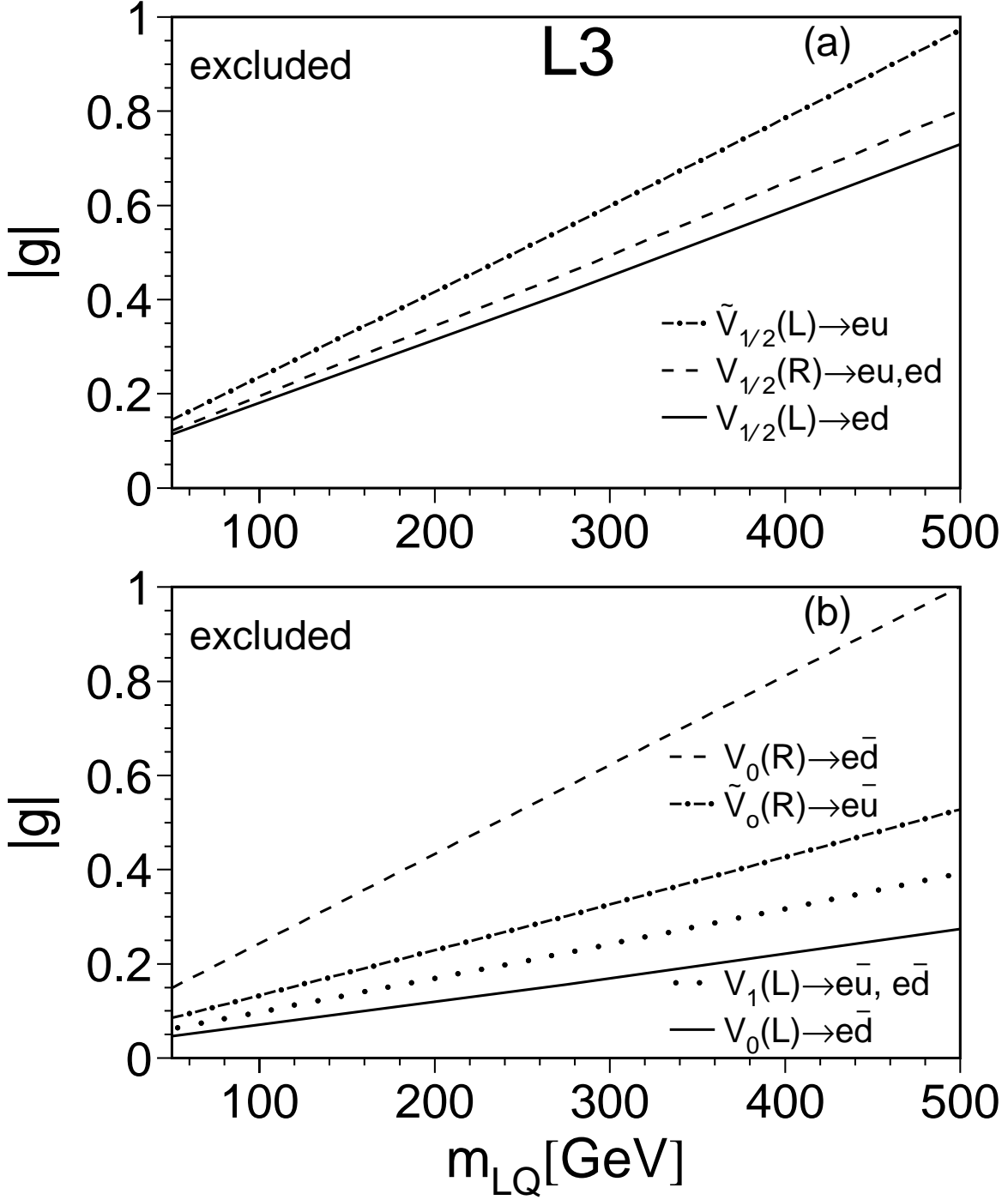
Figure 4: The 95% confidence level upper limits on |g_L| or |g_R| as a function of m_{LQ} for various vector leptoquarks derived from hadronic cross sections. Limits are shown for fermion number F=2 (a) and for F=0 (b).
