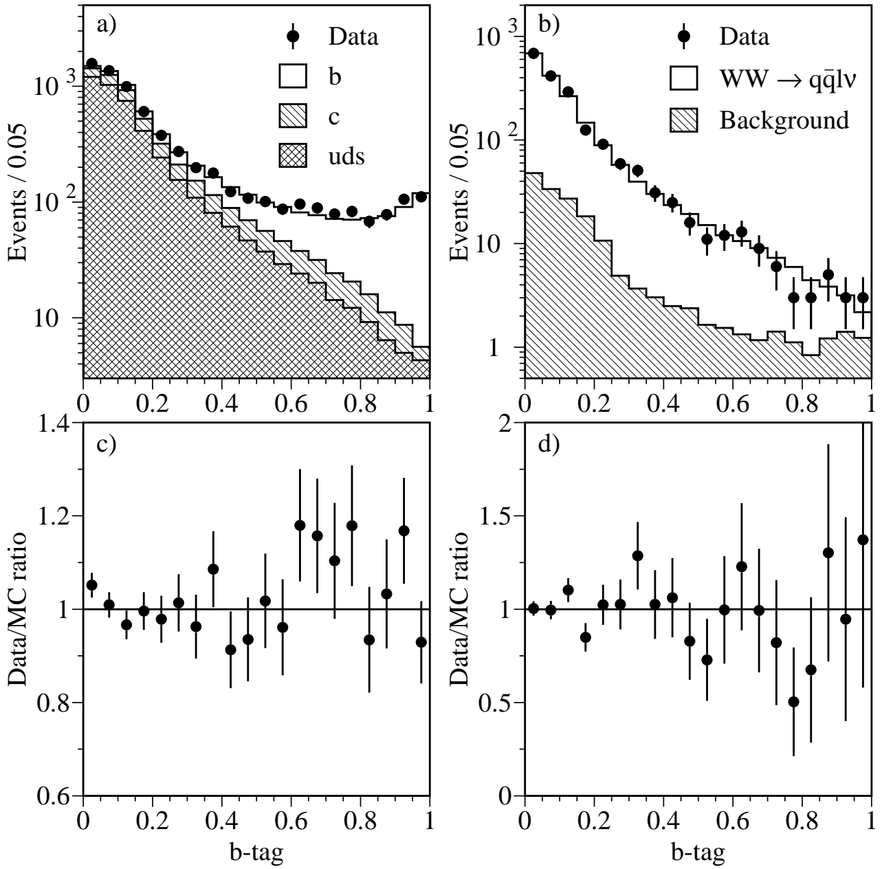
Figure 1: Distribution of the b-tag variable for jets in a sample of a) e^+e^- \rightarrow q\bar{q}(\gamma) and b) W^+W^- \rightarrow q\bar{q}l\nu events selected from the high-energy data collected in the year 2000. The data are compared to the simulation of Standard Model processes. The bin-by-bin ratio of the data to the simulated events is displayed in c) and d).
