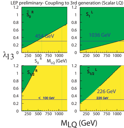
Figure 2: LEP preliminary exclusion plots for scalar LQ coupling to the 3rd generation of quarks.
