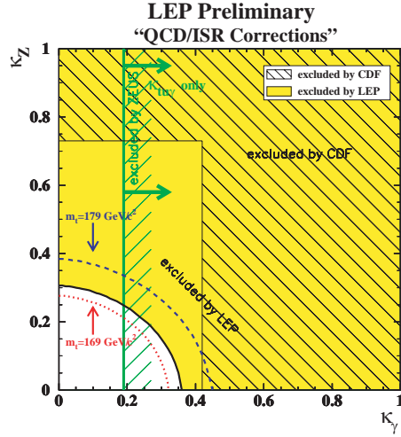
Figure 3: LEP combined limits on anomalous vertices \kappa_\gamma and \kappa_Z .
