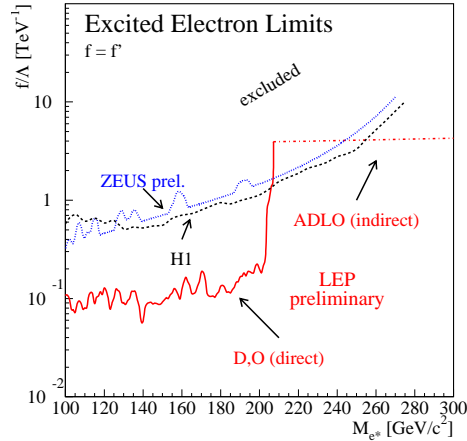
Figure 1: Limits on the mass vs coupling for the excited electron using combined direct and indirect search.
