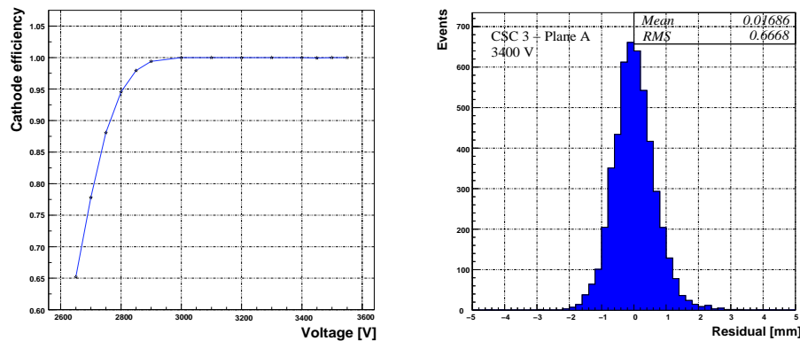
Fig. 16. Measurement of the efficiency of the TOTEM CSC detector as a function of the HV (left) and the spatial resolution (right).
