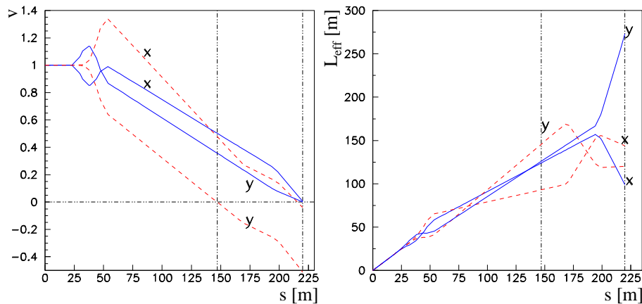
Fig. 2. Magnification v and effective length L_{eff} as a function of the distance from the IP (solid lines \beta^* = 1540 \text{ m} , dashed lines \beta^* = 1100 \text{ m} ).
