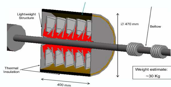
Fig. 17. The T2 telescope around the new CMS vacuum pipe.
