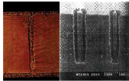
Fig. 12. Right: 290 \mu\text{m} deep C-shaped hole, filled with 2 \mu\text{m} polycrystalline silicon. The good quality of the etching and the uniformity of the deposition can be appreciated in the photo of a cut through the holes. Left: a cut wafer showing how the electrode looks after being filled with polysilicon.
