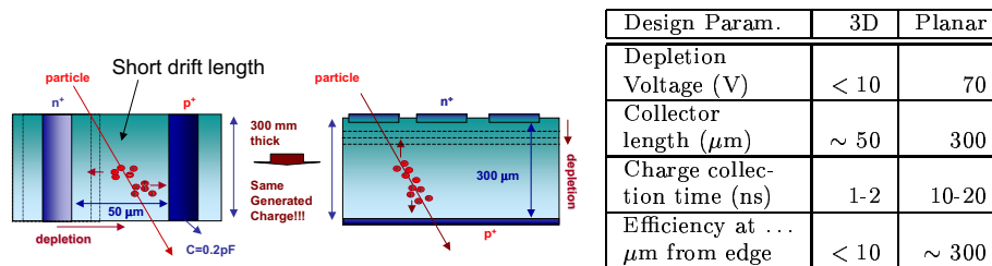
Fig. 13. A 3D detector design (left) compared to a standard planar detector (right). Table 2. Comparison of parameters
