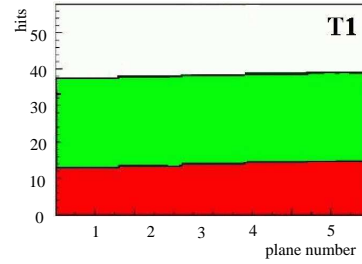
Fig. 19. Hits in the different detector planes of the TOTEM telescopes: the top line indicates the increase in the hit number due to the presence of the beam pipe.
