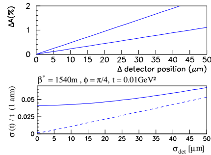
Fig. 6. (top) Acceptance uncertainty versus detector offset for t = 0.004 \text{ GeV}^2 (upper curve) and t = 0.01 \text{ GeV}^2 . (bottom) Relative t -resolution (1 arm only) versus detector resolution (solid), the dotted line shows the ideal case of zero beam divergence (lower curve).
