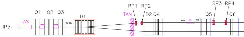
Fig. 3. The LHC beam line with the Roman Pots at 147 m and 220 m.
