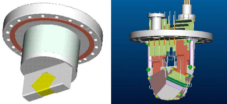
Fig. 7. A schematic view of the TOTEM Roman Pot detector system. The thin window separating the primary beam vacuum and the detector enclosure is seen at the bottom of the insertion. The detector arrangement with the front-end electronics and services is shown on the right.
