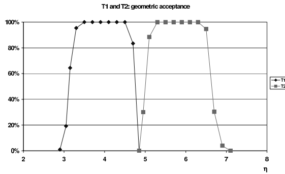
Fig. 18. Geometrical acceptance of T1 and T2.
