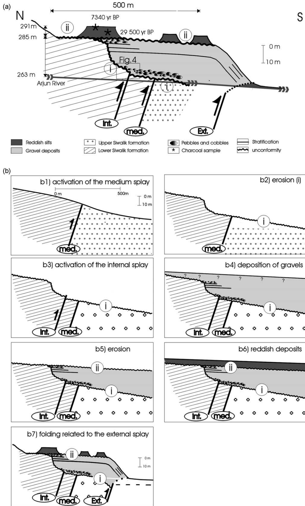
Fig. 3. (a) Sketch of the geomorphic, stratigraphic and thrust/sediment relationships along the Arjun Khola (A in Fig. 2); the vertical exaggeration is ~6, and graphically increases the dip of the faults; (int.) (med.) and (ext.) refer to the three splays of the MDT; (i) and (ii) refer to two distinct erosional surfaces. (b) Sketch of the kinematic evolution; (b1) the medium splay (2) is active; (b2) erosional surface (i) develops; (b3) the internal splay is active; (b4) gravels are deposited above the erosional surface (i), the internal splay and the medium splay; (b5) erosional surface (ii) develops before (b6) the deposition of the reddish silts; (b7) the external thrust (3) is active, all the previous structures are uplifted and the gravel deposits are folded above the external splay.
