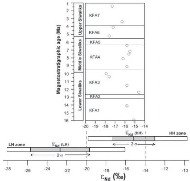
Fig. 5 Nd-isotope composition \epsilon_{\text{Nd}}(0) of samples from Siwalik sedimentary rocks of the Karnali River based on data from Huyghe et al. (2001) and new data (the present study). Along the base, the range of \epsilon_{\text{Nd}}(0) values from the Higher Himalayan (HH) zone and Lesser Himalayan (LH) zone from Robinson et al. (2001; and references therein) are shown with the average \epsilon_{\text{Nd}}(0) value marked with a black bar and the standard deviation of the average marked with gray bars. The limits of facies KFA1–KFA7 have been reported from their stratigraphic ages.
