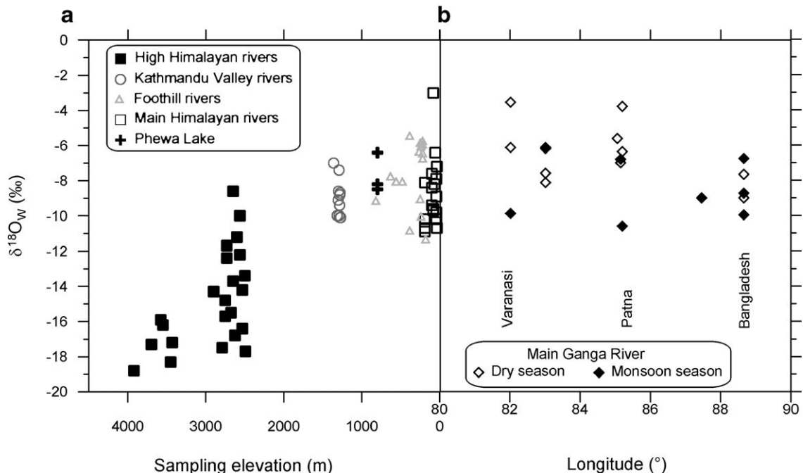
Fig. 3. \delta^{18}\text{O}_w values of the water samples as a function of: (a) sampling elevation for the High Himalayan rivers, Kathmandu Valley rivers, foothills and Main Himalayan rivers and Phewa Lake, and (b) longitude for the Main Ganga stream in the Ganga plain.
