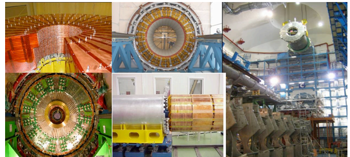
Fig. 7. Top left: 25 modules of the HEC wheel. Top middle: EM half-barrel in its cryostat. Bottom left: The HEC integration in its cryostat (behind the EM end cap). Bottom middle: insertion of the FCal in the cryostat. Right: lowering of the EM barrel cryostat to the ATLAS cavern.
