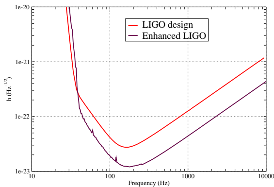
Figure 2. Enhanced LIGO sensitivity.
