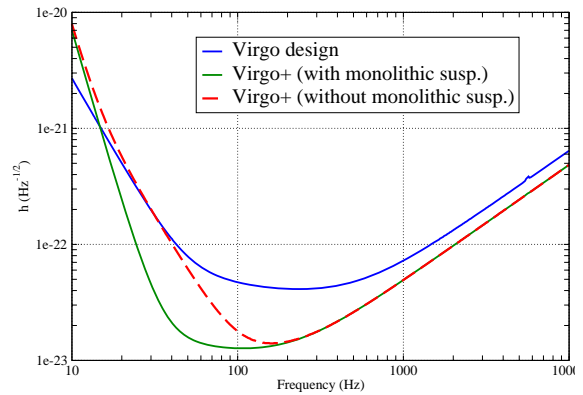
Figure 3. Virgo+ sensitivity.
