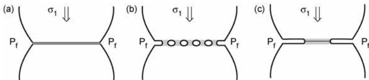
FIG. 11: Schematic illustrations of the 3 different PSC mechanisms. (a) “thin fluid film” model: thin adsorbed intergranular fluid film supports normal stress, with dissolution and diffusion occurring within the film. (b) “island-channel” model: multiple island structures separated by channels containing fluid at pore pressure; stressed islands dissolve preferentially until plastic or brittle failure occurs; alternatively, island structures may contain a trapped fluid film. (c) “free face and plastic deformation” model: dissolution occurs exclusively at free faces in pore fluid; once a critical stress is reached, the intergranular supporting ‘neck’ fails by plastic or brittle deformation, leading to compaction. Figure adapted from [60].
