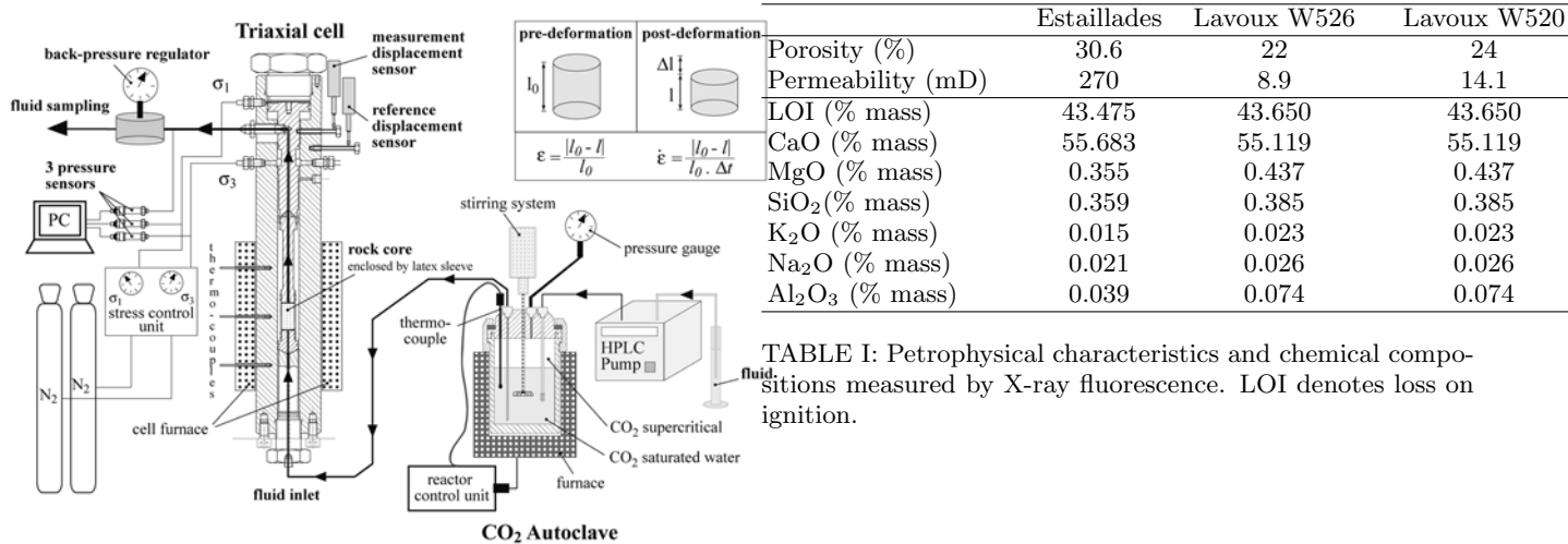
FIG. 1: Triaxial cell used for measuring axial strain in presence H 2 O-CO 2 fluids. Vertical stress \sigma_1 , lateral stress \sigma_3 ( =\sigma_2 ), temperature, fluid pressure P_f , and injection rate were all separately controlled and measured. High P CO 2 fluids were prepared in separate autoclave. Inset shows expressions for strain, \epsilon and strain rate, \dot{\epsilon} .
