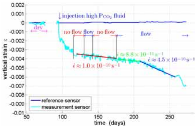
FIG. 5: Vertical axial strain deformation measured for Lavoux W526 sample in the absence of fluid and during injection of high P_{CO_2} saline fluid (cyan curve). Time periods with no data represent non-stable conditions associated with parameter changes. The red time period \dot{\epsilon} includes a short flow period. Note that the renewed injection of high P_{CO_2} saline solution caused a large increase in \dot{\epsilon} , but after time lag of \approx 40 days. The end of the experiment was marked by a sudden, rapid increase in strain and strain rate.
