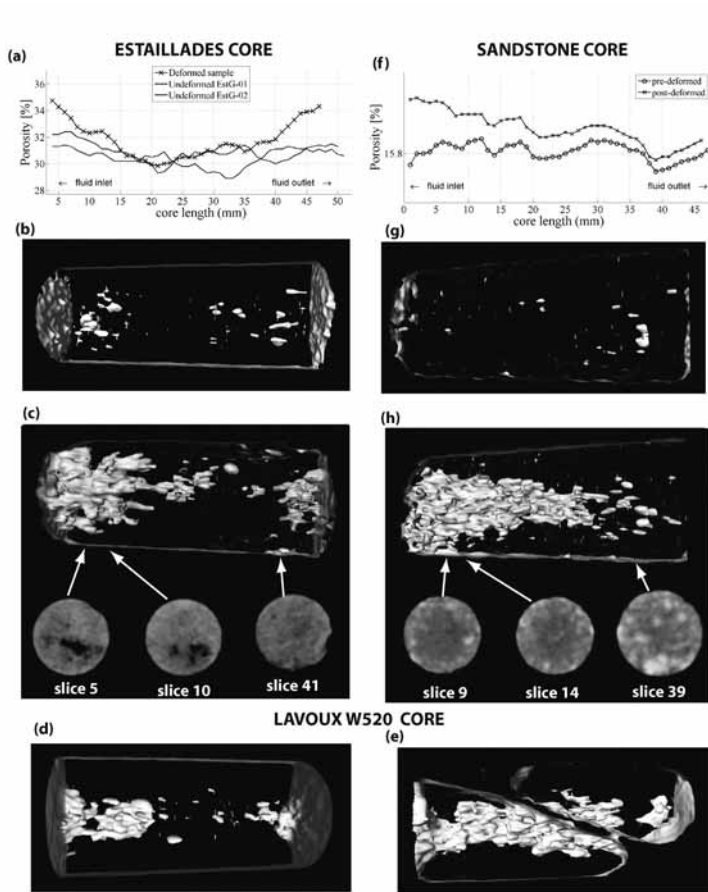
FIG. 9: X-ray computed tomography (CT) profiles and images of samples before and after deformation. All core lengths equaled 45-50 mm. (a) CT-based porosity profile of deformed Estaillasses limestone, compared to 2 different undeformed samples. Note elevated porosities in inlet and outlet regions after deformation. (b) CT image (1600 attenuation) of an Estaillasses limestone before deformation (corresponds to porosity profile EstG-02 in (a)). (c) CT image (1600 attenuation) of deformed Estaillasses limestone (different sample than in (b)). Note CT density slices and locations in core, porous channel-like regions appear black in slices 5 and 10. (d) CT image (1965 attenuation) of Lavoux W520 before deformation. (e) CT image (1965 attenuation) of same Lavoux W520 after deformation. Note development of axial porosity. Non-continuity of sample due to post-experiment shear damage. (f) CT-based porosity profile of sandstone before and after deformation. Pre-deformation porosity based on independent measurement, post-deformation porosity cannot be quantified due to lack of CT calibration. (g) CT image (1290 attenuation) of sandstone before deformation. (h) CT image (1290 attenuation) of same sandstone after deformation, showing extensive axial porosity development. Note CT density slices and locations in core.
