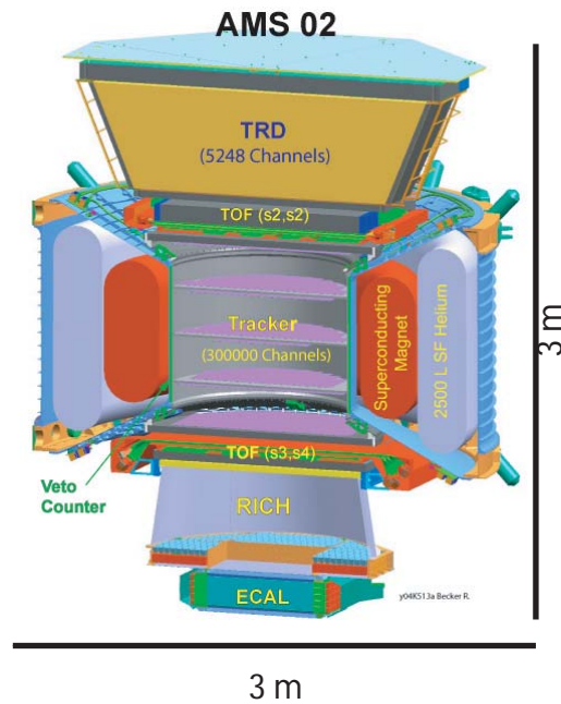
Figure 1. Schematic view of the AMS detector.
