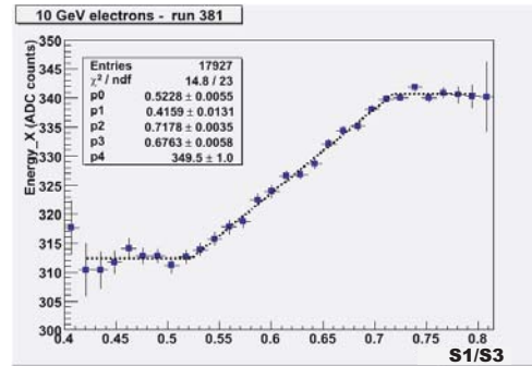
Figure 14. Dependance of the energy as a function of S1/S3 (See text).
