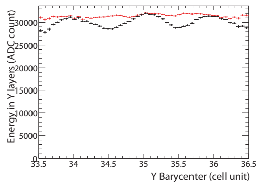
Figure 16. Energy before (black) and after (grey/red) impact correction.
