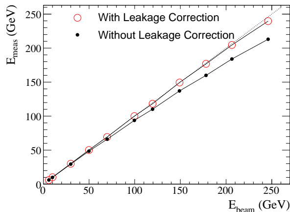
Figure 19. Energy before and after leakage correction in function of the beam energy.
