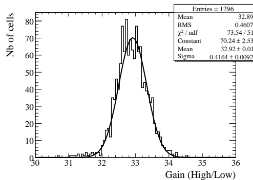
Figure 9. Distribution of the PMTs' gains measured in test beam.
