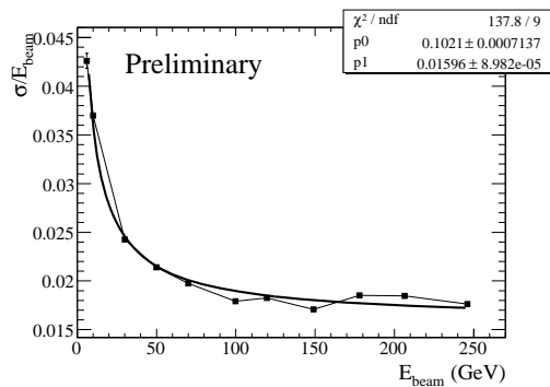
Figure 20. Preliminary results on the energy resolution.
