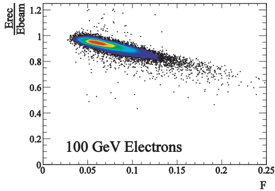
Figure 17. Example of the linear dependence of the relative leakage energy, given by the ratio of the reconstructed energy E_{rec} , (including all preceding corrections) over the beam energy as a function of F , the fraction of energy in the last two layers for 100 GeV Electrons
