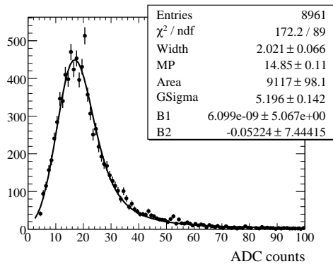
Figure 6. Example a MIP distribution fitted with a Landau convoluted by a Gaussian function + an exponential background,
