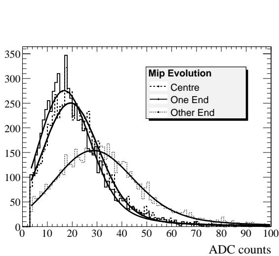
Figure 11. MIP signal measured at three different positions along the fiber.
