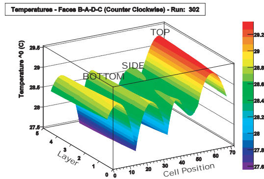
Figure 4. Map of the extrapolated temperatures on each face on the calorimeter.
