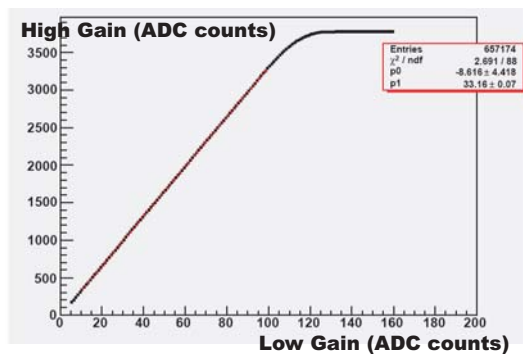
Figure 8. Relation between High to Low gain for a single anode.
