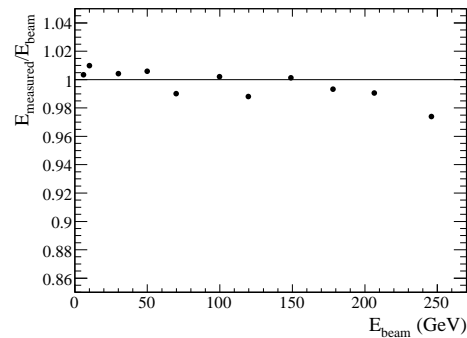
Figure 21. Preliminary result on the linearity.
