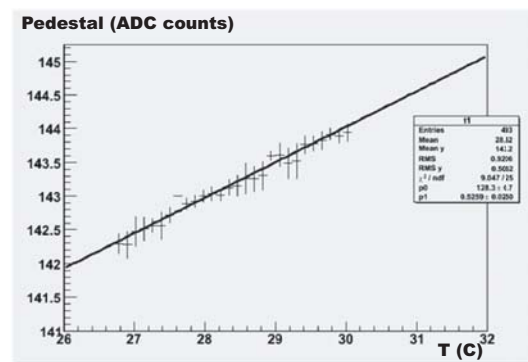
Figure 5. A typical dependence of the pedestal as a function of the temperature.
