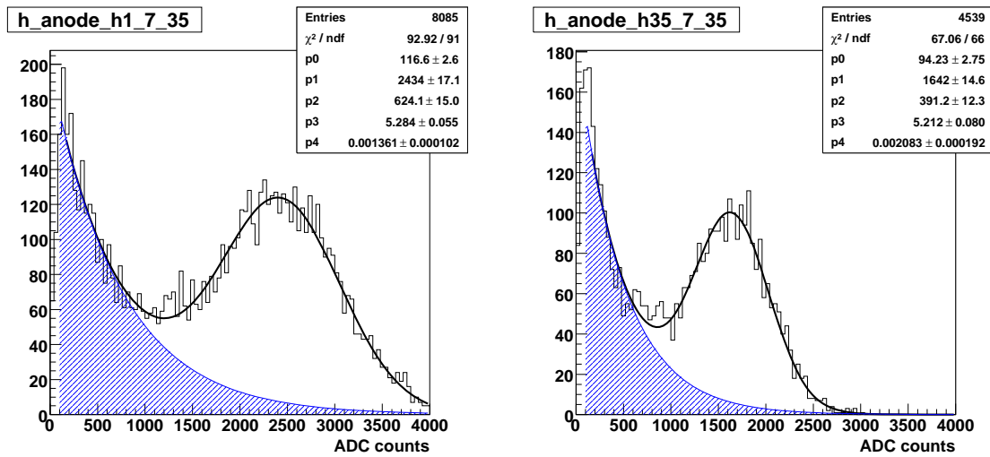
Figure 10. 10 GeV Electron signal measured close (left) and far (right) from the photomultiplier.
