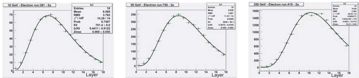
Figure 22. Longitudinal electromagnetic profiles fitted from left to right at the energies of 10, 50 and 250 GeV.
