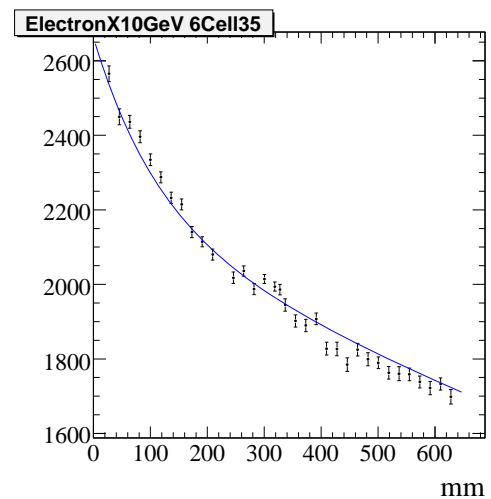
Figure 12. Example of fit of the attenuation.
