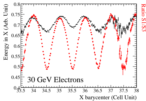
Figure 13. Sensitivity of the energy reconstruction to the impact position given by the barycenter (small black dots), Sensitivity of the ratio S1/S3 (See text) to the impact position (large red dots)
