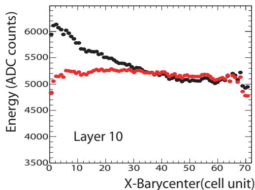
Figure 15. Energy measured in layer 10 before (black) and after (grey/red) correcting for the attenuation as a function of the X position.
