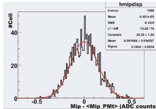
Figure 7. Dispersion of MIPs within PMTs observed in test beam.
