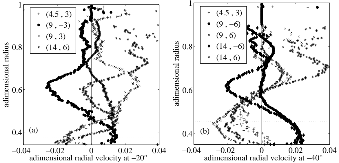
Fig. 12. Radial velocity, obtained by ultrasonic Doppler velocimetry, as a function of adimensional radius (vertical axis) at two different latitudes: -20^\circ (a) and -40^\circ (b). The dotted line indicates the radius of the tangent cylinder on the inner sphere, whose adimensional radius is 0.35 (bottom of the plots). All velocities are normalized with the differential tangential velocity at the equator of the inner sphere. The profiles are labelled by their (f, \Delta f) pair. Note that the sign of the radial velocity changes as the sign of \Delta f , as expected for Ekman-pumping dominated flow.
