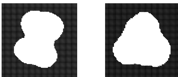
FIG. 8. \lambda_5 (left) and \lambda_6 (right)
