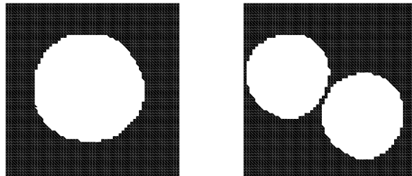
FIG. 6. \lambda_1 (left) and \lambda_2 (right)
