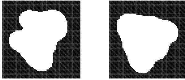
FIG. 10. \lambda_9 (left) and \lambda_{10} (right)
