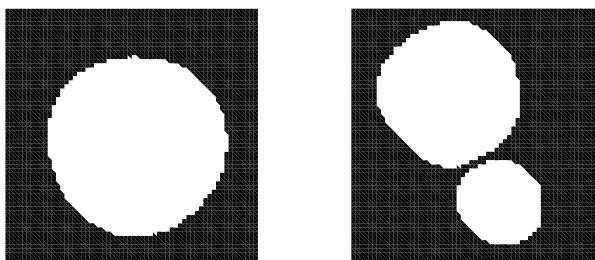
FIG. 7. \lambda_3 (left) and \lambda_4 (right)
