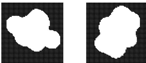
FIG. 9. \lambda_7 (left) and \lambda_8 (right)
