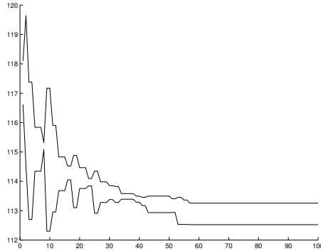
FIG. 4. Evolution of \lambda_3 and \lambda_4
