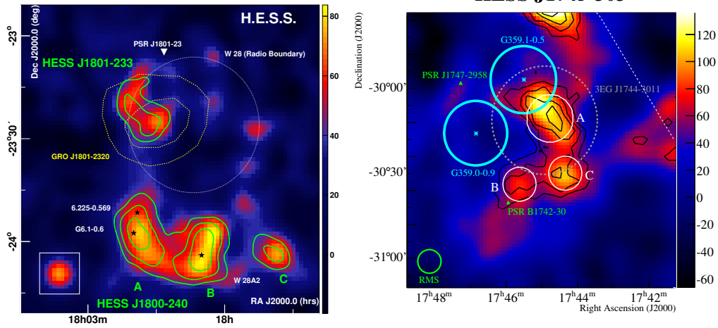
Figure 1: Left : H.E.S.S. \gamma -ray excess map Gaussian smoothed ( \sigma=4.2' ), with 4\sigma to 6\sigma significance contours overlaid. Several objects are indicated: SNR W 28 radio boundaries (thin-dashed circle), HII regions (black stars), PSR J1801-23 (white triangle), GRO J1801-2320 (dashed yellow lines - 68% and 95% position confidence levels). The inset shows the H.E.S.S. point spread function. Right : H.E.S.S. excess map Gaussian smoothed ( \sigma=0.07^\circ ) of HESS J1745-303 with 4\sigma to 7\sigma statistical significance contours overlaid in black. The dashed circle is the 95% error circle for the location of 3EG J1744-3011. The Galactic plane is marked with a dotted line.
