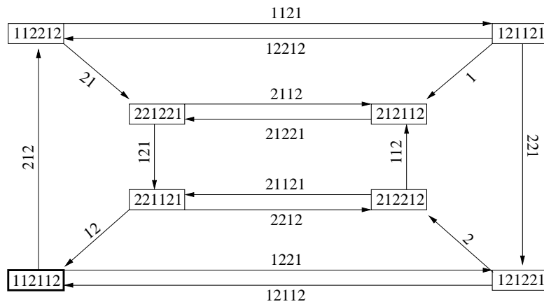
Fig. 4: Reduced 6-order De Bruijn graph of m
