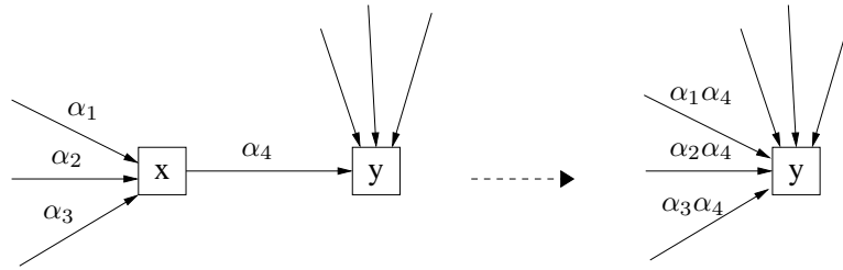
Fig. 1: Edge reduction in the De Bruijn graph
