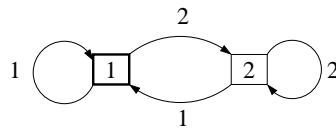
Fig. 3: Naive algorithm
