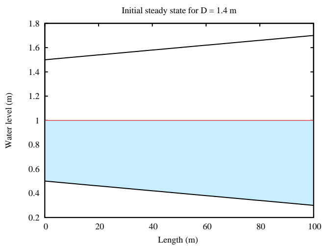
Figure 18: Initial still water steady state for contracting, uniform and expanding pipes .
