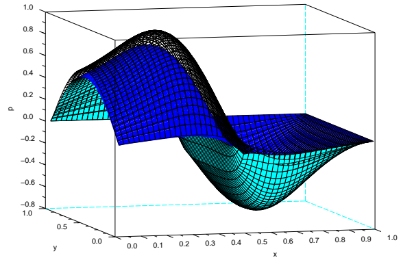
Figure 4: On the left figure, we indicate the part of the top boundary which is rough. On the right figure, we compare the pressure profile without rugosity (grid) and the pressure profile obtain with the corresponding rugosities (plain).
