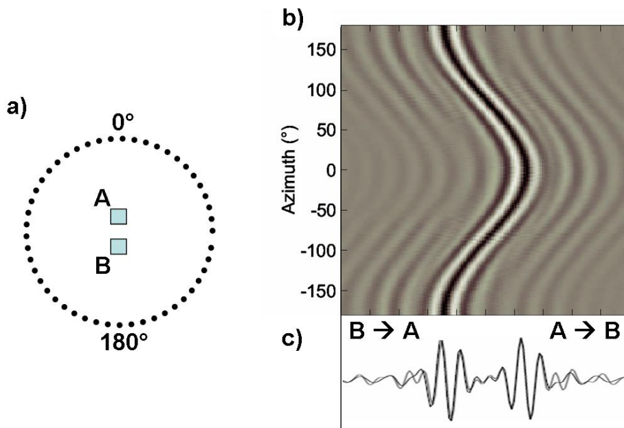
FIG. 1.24 – Interpretation of the convergence of the correlation towards the Green's function with the stationary phase theorem. Modified from Gouédard (2008). a) Schematic representation of the 2 receivers A and B, and the uniformly distributed sources around the receiver pair. b) Cross-correlations computed for all sources plotted versus azimuth. c) The sum of all source contributions (black) is equal to the theoretical Green's function (grey).
