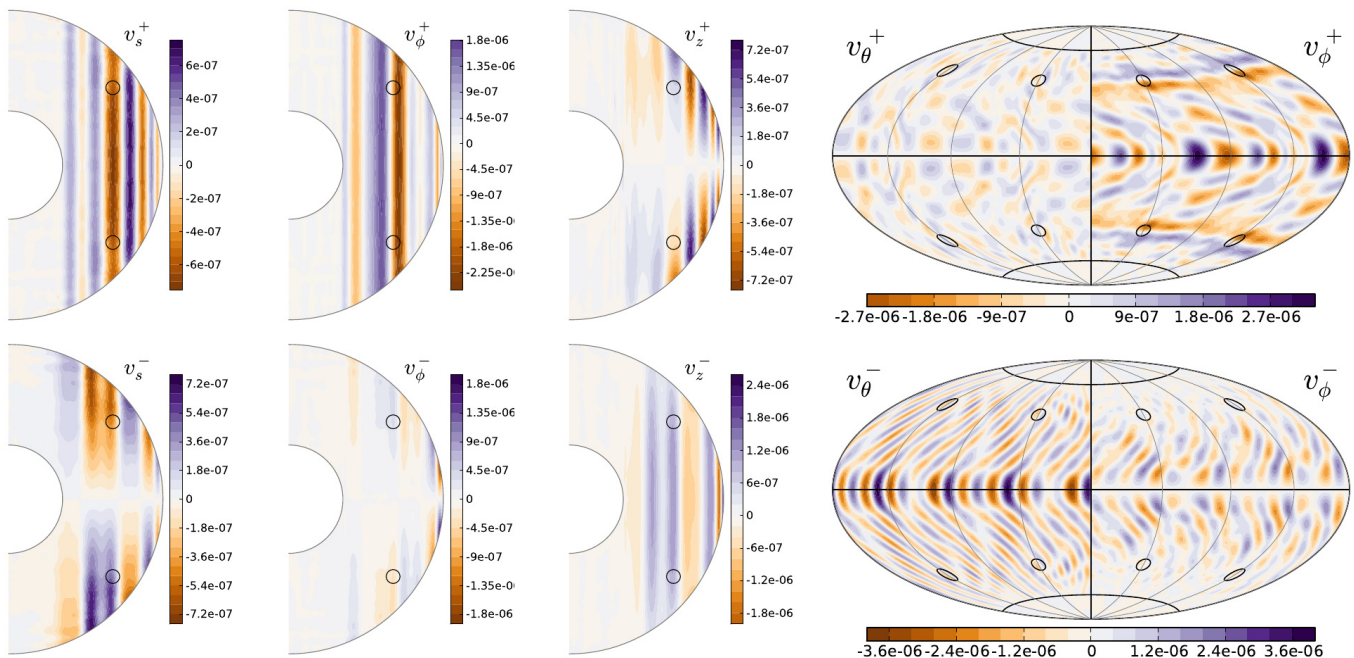
FIG. 1. Flows resulting from a symmetric (top) or anti-symmetric (bottom) forcing followed by 110T of free decay. From left to right: the cylindrical components ( v_s, v_\phi, v_z ) in the meridional plane containing \mathbf{r}_\pm , and the spherical components ( v_\theta, v_\phi ) at the core-surface (note on the right the use of a 4-fold symmetry in the simulation). The circles indicate the location of the applied forcing in the meridian plots, and its projection along the z -axis on the surface plots. The surface projection of the equator of the inner-core is also drawn. Velocities are expressed in units of a\Omega .
