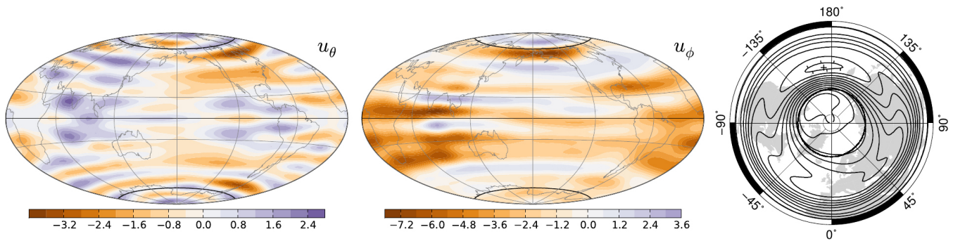
FIG. 3. Inverted flow \bar{\mathbf{u}}^\pm using \lambda_A = 8 \times 10^6 averaged over the CHAOS-3 era. From left to right : u_\theta and u_\phi components in km/yr, and the stream-function \xi of the symmetric part \bar{\mathbf{u}}^+ viewed from north-pole defined by \bar{\mathbf{u}}^+ = (\cos\theta)^{-2} \mathbf{r} \times \nabla\xi . The parallel corresponding to the trace of the TC is drawn (as well as \pm 20^\circ , related to table IV).
