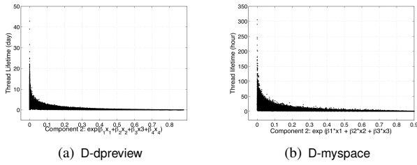
Figure 6: risk factor component ( x_1\beta_1 \dots x_k\beta_k ) vs. the lifetime of threads
