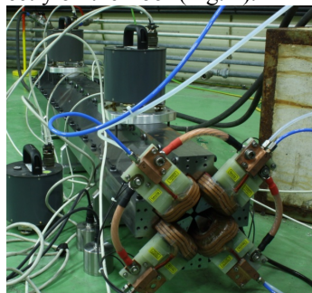
Figure 2: Water cooling measurements with the magnet on equivalent supports on the floor
