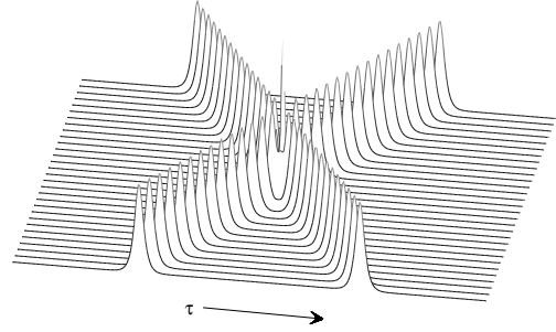
Figure 5. Elastic collision of two NLS solitary waves traveling at the same speed s = 2 , for \mu = 2 .
