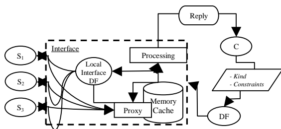
Fig.4. Advanced Interface architecture.
