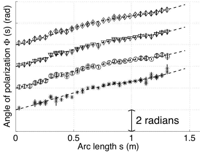
Figure 5: Measured geometric phase as a function of arc length along the helix for signals filtered at 1.4 kHz, 2.5 kHz, 4.0 kHz and 5.8 kHz. The dashed line represents the linear regression with correction for the coupling and orthogonality of the accelerometers. The origins of the curves are arbitrary.
