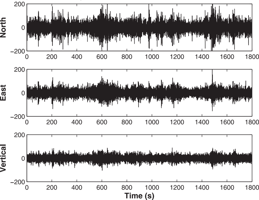
Example of tremor recorded March 21, 2005
