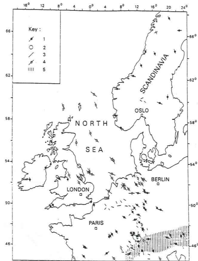
Compilation of observed maximum horizontal present-day stress directions in the Northwest European Platform. 1 = direction of maximum horizontal stress from in-situ stress measurements. 2 = a horizontal stress equal in all directions as found in in-situ stress measurements. 3 = the direction of maximum horizontal stress inferred from earthquake focal-mechanism studies. 4 = the direction of maximum horizontal stress inferred from break-out analysis. 5 = Alpine fold belt. The data indicate stress propagation away from the Alpine fold belt in the platform region. (After Klein and Barr, 1986.)
