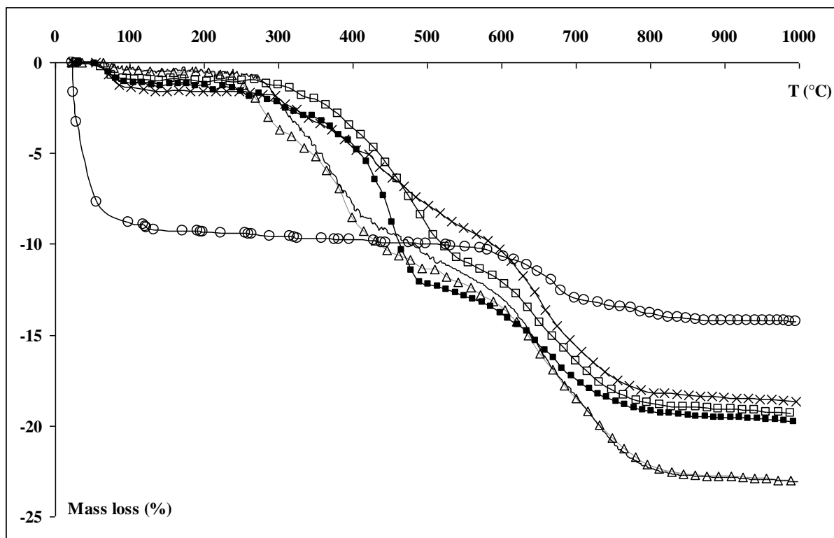
Figure 3 : TGA curves of montmorillonite samples : raw (O) and after adsorption of BMIImCl (□), OMImCl (no symbol, full line), OPyBr (Δ), BPyBr (■) and AMImCl (×).
