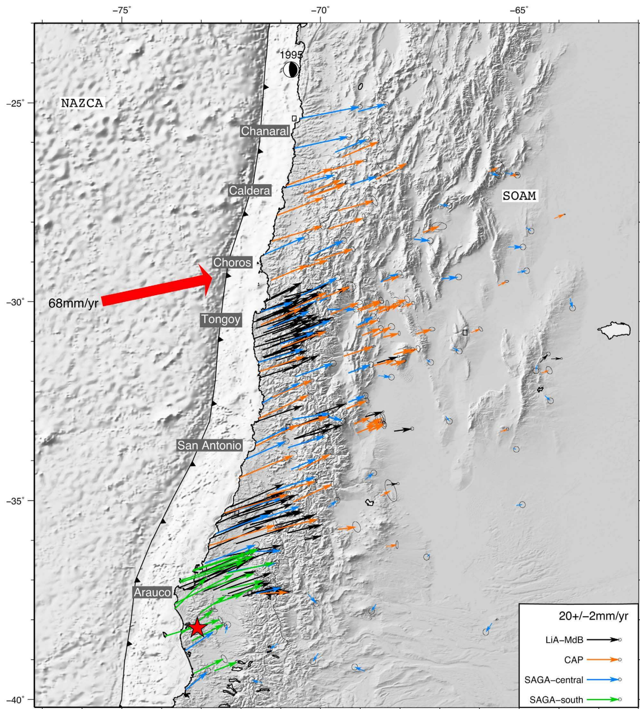
Figure 3. Final compiled data set of the upper-plate interseismic surface deformation relative to a fixed South-American plate defined by the NNR-NuvelIA model. Different colors depict different data sets (detailed in Table S3 in Text S2 of the auxiliary material). LiA-MdB [Ruegg et al. , 2009; Vigny et al. , 2009]; CAP [Bevis et al. , 1999; Brooks et al. , 2003]; SAGA-central [Khazaradze and Klotz, 2003; Klotz et al. , 2001]; SAGA-south [Moreno et al. , 2008]. The hypocenter of the 1960 M_w 9.5 Valdivia earthquake is plotted as a red star. The CMT focal mechanism of the 1995 Antofagasta earthquake is plotted as a beach ball. The bold red arrow shows the Nazca plate convergence with respect to the stable South America (68 mm/yr). Major coastal features are named in gray rectangles.
