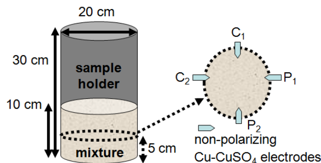
Figure 1: Illustration of the sample holder dimensions used for the measurement
